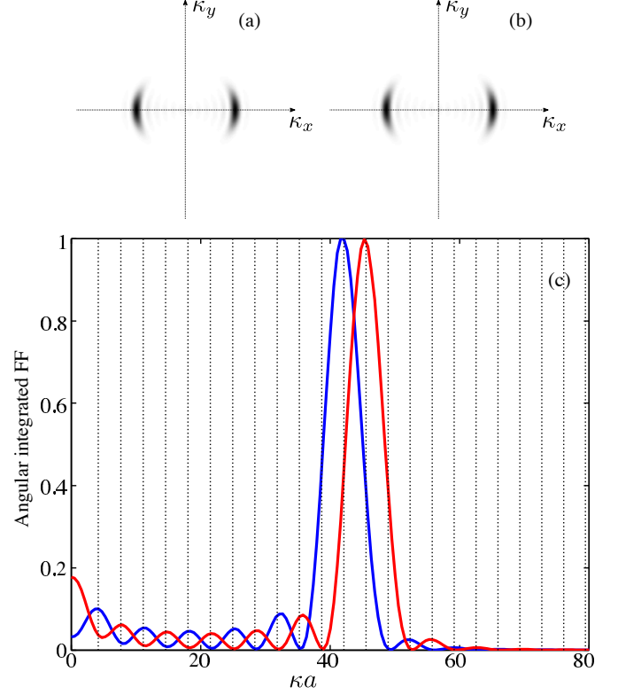
FIG. 15. (a,b) Numerical FF calculated for two different 2-PO regular modes with p = 12 and p = 13 respectively. (c) Angular integrated FFs. Blue line corresponds to case (a) and red line to case (b). The vertical dashed lines correspond to the value of the wavenumber of the u_{0,p} modes.
