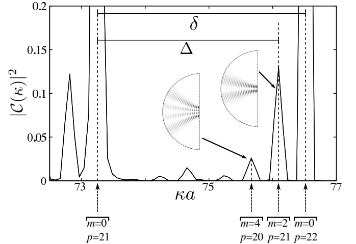
FIG. 12. Zoom of the spectrum of Fig. 11(f) between two peaks p = 21 and p = 22 . In inset, the intensity of the modes corresponding to u_{4,20} and u_{2,21} .
