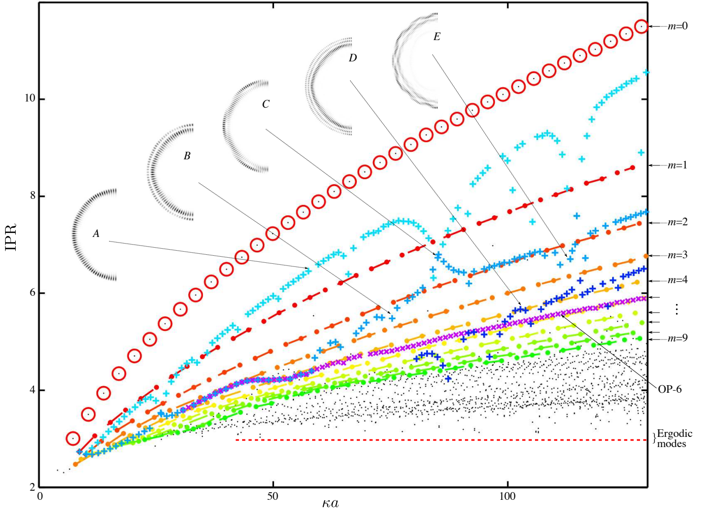
FIG. 8. Inverse Participation Ratio (IPR) as a function of the transverse wave number \kappa a for the mixed case ( \gamma = 0.95 ) ; Families of modes are distinguishable as shown by the different markers: red circles \circ correspond to 2-PO regular modes, from red to green dots [from \bullet to \bullet ] correspond to higher order regular modes denoted from m = 1 to m = 9 , purple crosses \times correspond to modes built on the 6-PO, light, medium and dark blue crosses + , + and + correspond to whispering gallery modes (insets A to E).
