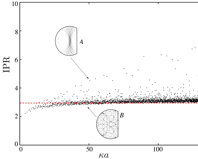
FIG. 7. Inverse Participation Ratio (IPR) as a function of the transverse wave number \kappa a for the chaotic case ( \gamma = 3/2 ); As expected, the IPR concentrates in the vicinity of \text{IPR}=3 except for the modes built on neutral orbits (upper inset, A). Inset B shows a generic ergodic mode.
