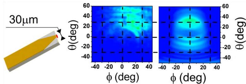
Fig 5. Simulated (right) and measured (left) far-field patterns of a 3-mm-long 80- \mu\text{m} -wide metal-metal THz QCLs with a 250- \mu\text{m} -long inverse planar horn structures. The measurements were all taken at 77 K.
