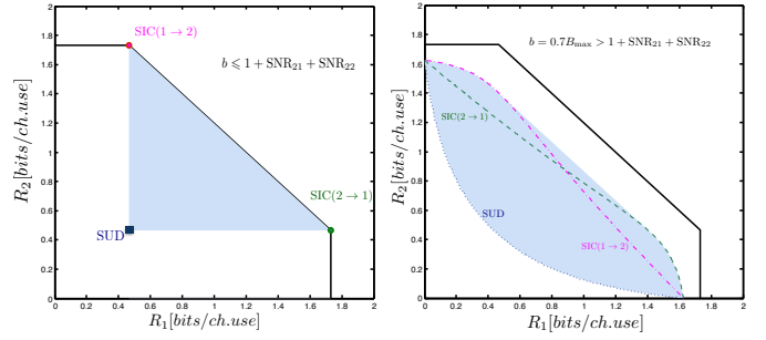
Fig. 1. Projection of the sets \mathcal{N}_{\text{SUD}}(b) and \mathcal{N}_{\text{SIC}(i \rightarrow j)}(b) over the R_1 - R_2 plane for different values of b . The information capacity region is also plotted as a reference (white region inside solid lines) for \text{SNR}_{11} = \text{SNR}_{12} = \text{SNR}_{21} = \text{SNR}_{22} = 10 . The blue region is the convex hull of \mathcal{N}_{\text{SUD}}(b) \cup \mathcal{N}_{\text{SIC}(1 \rightarrow 2)}(b) \cup \mathcal{N}_{\text{SIC}(2 \rightarrow 1)}(b) .
