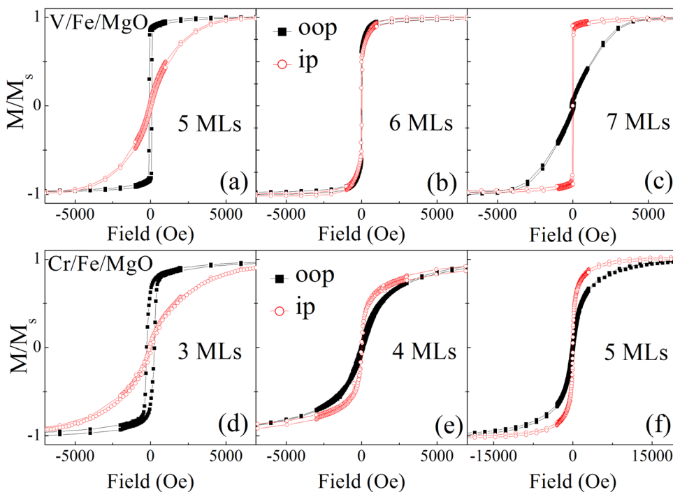
FIG. 2. Room temperature normalized magnetization as a function of magnetic field applied out-of-plane (OOP-black squares) and in the film plane (IP-red open circles), measured on V/Fe/MgO sample with t_{\text{Fe}} set to (a) 5 MLs, (b) 6 MLs and (c) 7 MLs and on Cr/Fe/MgO with t_{\text{Fe}} set to (d) 3 MLs, (e) 4 MLs and (f) 5 MLs.
