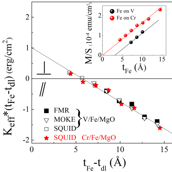
FIG. 3. Effective anisotropy constant K_{\text{eff}} times t_{\text{Fe}} - t_{\text{dl}} as a function of t_{\text{Fe}} - t_{\text{dl}} deduced from SQUID-VSM, FMR, and MOKE measurements at RT for both V/Fe/MgO and Cr/Fe/MgO systems. The line is a fit using Eq. (2). In inset are plotted the areal magnetization versus Fe thickness, showing that t_{\text{dl}} = 0 for Fe on Cr and t_{\text{dl}} = 3 \text{ \AA} for Fe on V.
