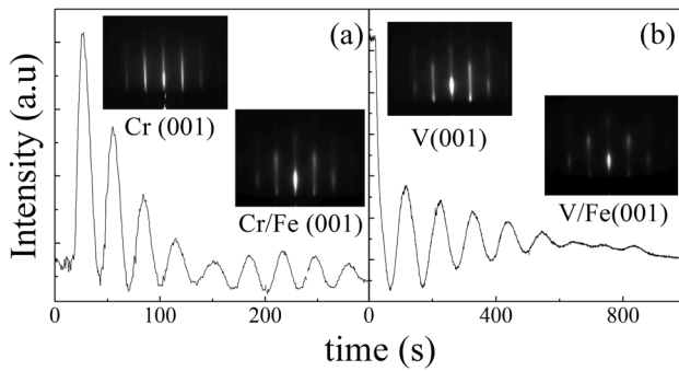
FIG. 1. RHEED intensity oscillations recorded during the growth of Fe on Cr(001) (a) and V(001) (b), respectively. In inset, RHEED patterns of V and Cr (001) buffer layers are shown, as well as Cr/Fe(8 MLs) and V/Fe(8 MLs).
