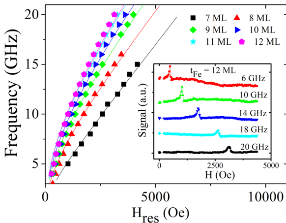
FIG. 4. FMR resonance field plotted versus DC magnetic field frequency (points) and simulations (lines) performed on V/Fe/MgO wedge with t_{\text{Fe}} = 7, 8, 9, 10, 11, and 12 \text{ MLs} . In inset, typical FMR responses versus field for t_{\text{Fe}} = 12 \text{ MLs} for several excitation frequencies of the in-plane applied DC field.
