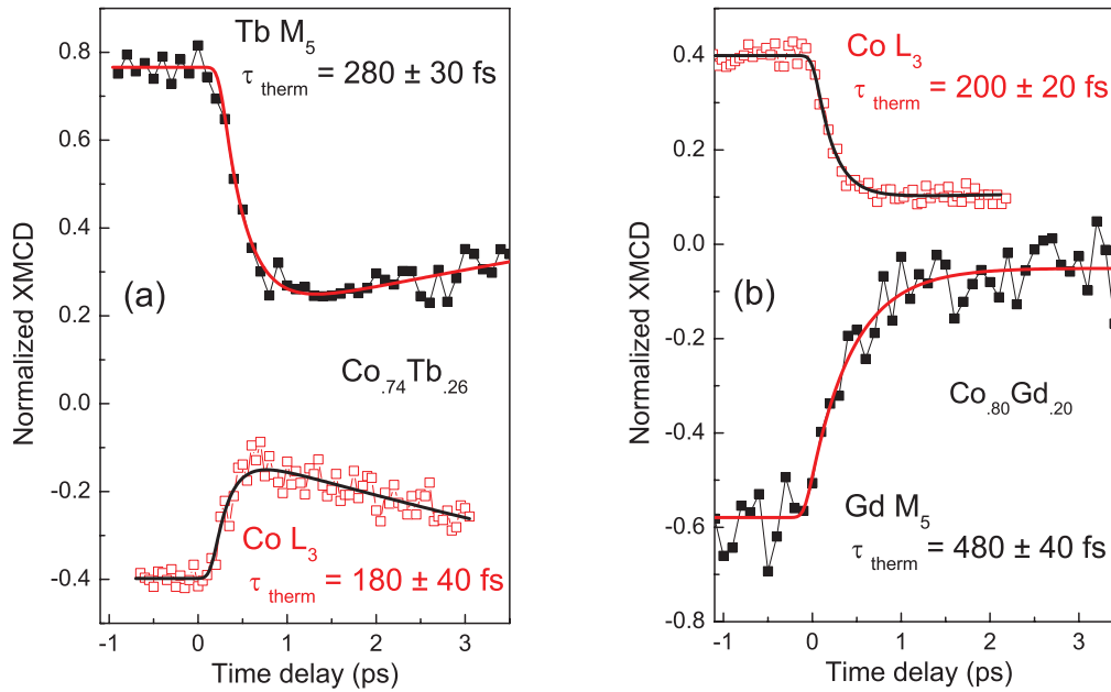
FIG. 3. (Color online) Ultrafast dynamics of (a) Co L_3 , Tb M_5 for the \text{Co}_{0.74}\text{Tb}_{0.26} alloy and (b) Co L_3 , Gd M_5 edges for the \text{Co}_{0.80}\text{Gd}_{0.20} alloy. The respective simulations obtained by approximating the rate equations of the two-temperature model are superposed as smooth lines. For the sample \text{Co}_{0.74}\text{Tb}_{0.26} the best fits are obtained for \tau_{\text{therm}} = 280 \pm 30 fs at the Tb M_5 edge and \tau_{\text{therm}} = 180 \pm 40 fs at the Co L_3 edge. For the sample \text{Co}_{0.80}\text{Gd}_{0.20} the best fits are obtained for \tau_{\text{therm}} = 480 \pm 40 fs at the Gd M_5 edge and \tau_{\text{therm}} = 200 \pm 20 fs at the Co L_3 edge. The XMCD values at the working temperature ( t < t_0 ) are provided by using the XMCD data at the Co L_3 , Tb M_5 , and Gd M_5 edges from the static measurements as given in Fig. 1. The working temperature of the sample \text{Co}_{0.74}\text{Tb}_{0.26} is T = 400 K, whereas T_{\text{comp}} = 550 K. The working temperature of \text{Co}_{0.80}\text{Gd}_{0.20} is T = 290 K, whereas T_C = 450 K. During the pump-probe experiments, close values of laser fluences were used ( 8\text{--}12 mJ/cm ^2 ), corresponding to close temperature intervals between working temperatures and the laser-excited-state temperatures where ultrafast demagnetization is observed.
