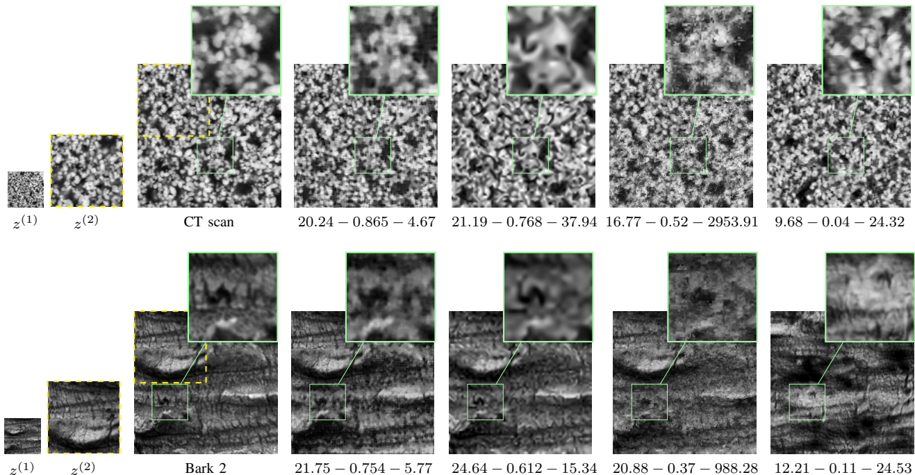
Fig. 7. PSNR – SSIM – Err x . From the left to the right: low-resolution image (down-sampling factor r = 4 , noise standard deviation \tau = 10 , blur 3 \times 3 ), high-resolution patch (25% of the total image), true image, proposed approach, Dong et al. [64], Hertzmann et al. [34] and Portilla et al. [65].
