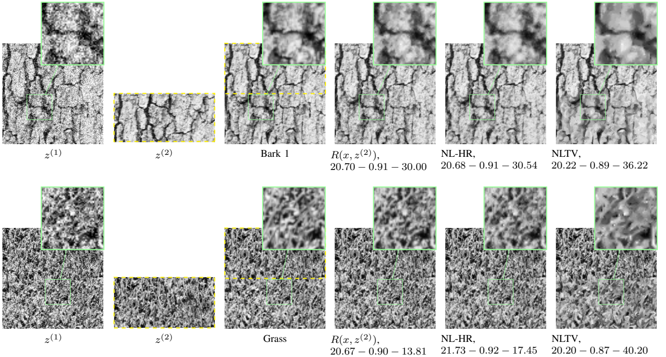
Fig. 5. \text{PSNR} - \text{SSIM} - \text{Err}_{\bar{x}} . From the left to the right: noisy image (noise standard deviation \tau = 50 ), high-resolution patch (50% of the total image), true image and the results of: the proposed nonlocal regularization, the nonlocal regularization of [46], and the classical NLTV [28].
