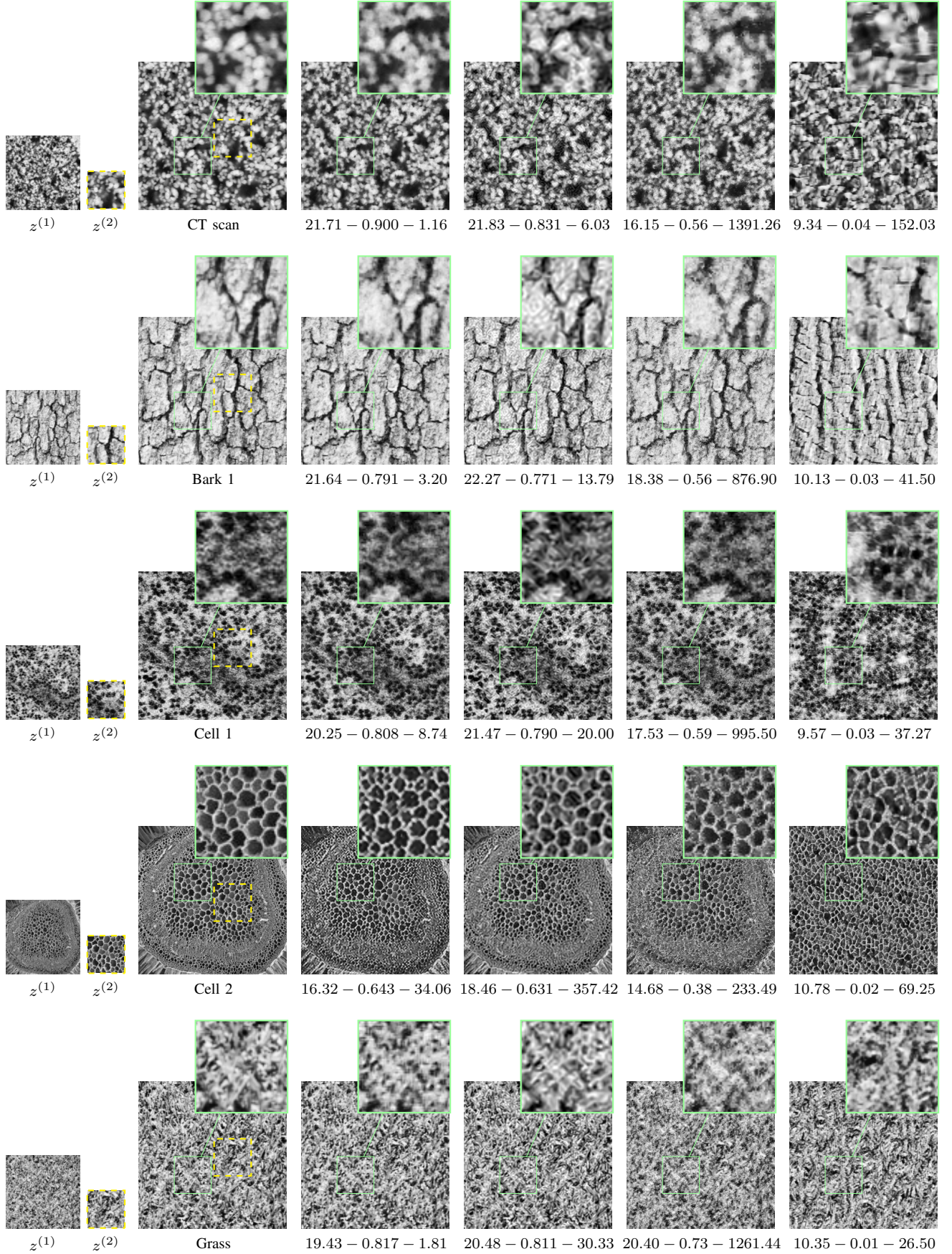
Fig. 8. PSNR – SSIM – Err x . From the left to the right: low-resolution image (down-sampling factor r = 2 , noise standard deviation \tau = 10 , blur 3 \times 3 ), high-resolution patch (6.25% of the total image), true image, proposed approach, Dong et al. [64], Hertzmann et al. [34] and Portilla et al. [65].
