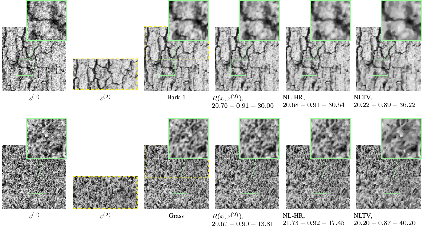
Fig. 5. PSNR – SSIM – \text{Err}_x . From the left to the right: noisy image (noise standard deviation \tau = 50 ), high-resolution patch (50% of the total image), true image and the results of: the proposed nonlocal regularization, the nonlocal regularization of [46], and the classical NLTV [28].
