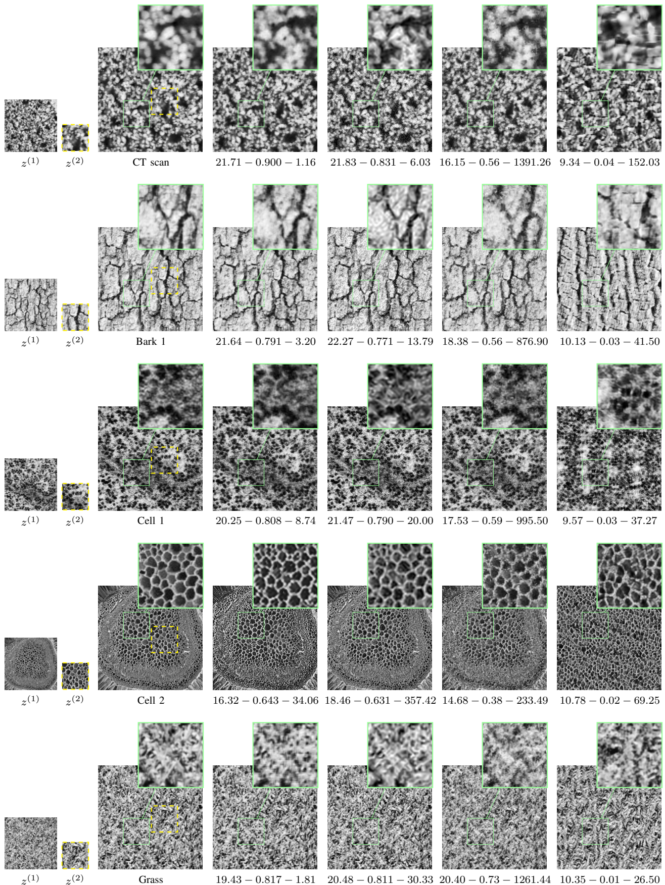
Fig. 8. PSNR - SSIM - Err \bar{x} . From the left to the right: low-resolution image (down-sampling factor r = 2 , noise standard deviation \tau = 10 , blur 3 \times 3 ), high-resolution patch (6.25% of the total image), true image, proposed approach, Dong et al. [64], Hertzmann et al. [34] and Portilla et al. [65].
