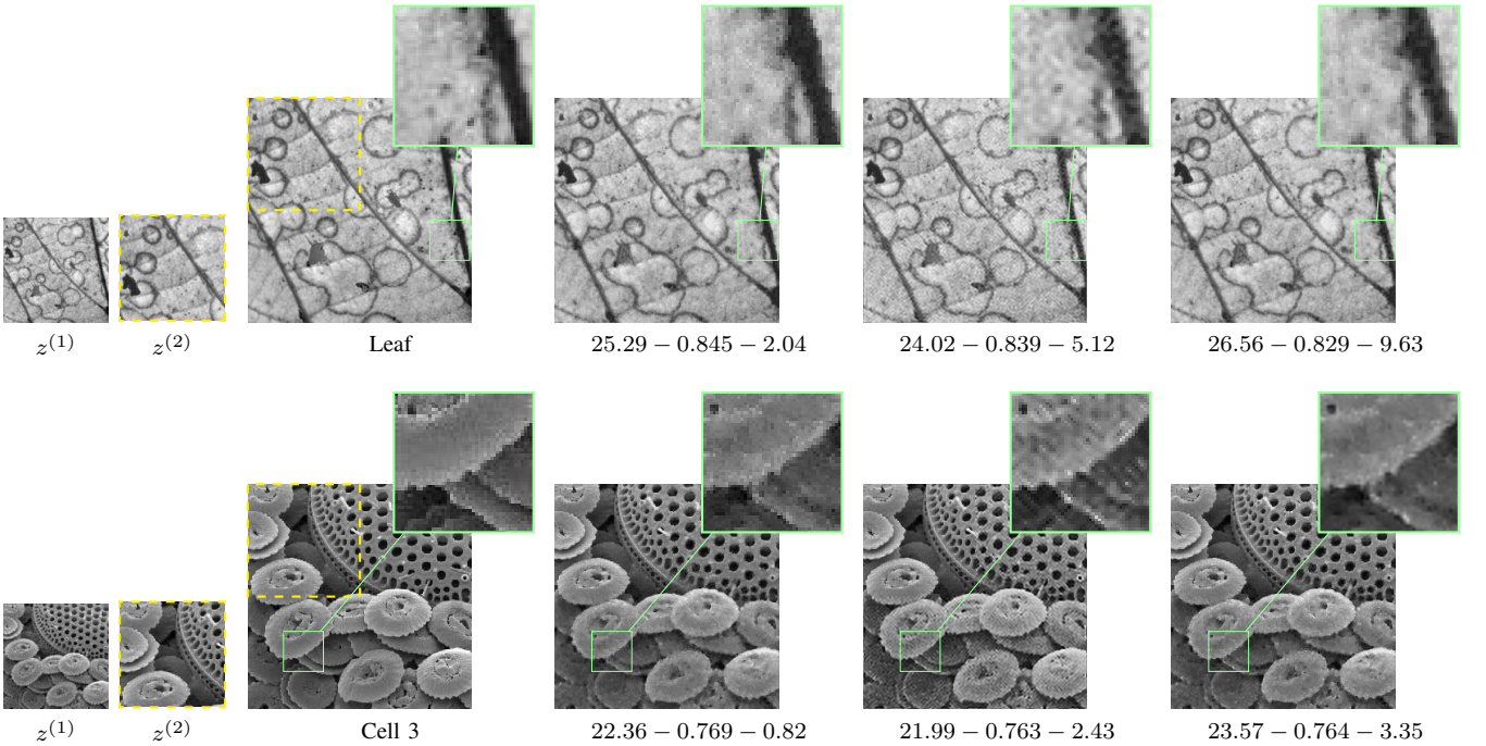
Fig. 6. PSNR - SSIM - Err \bar{x} . From the left to the right: low-resolution image (down-sampling factor r = 2 , noise standard deviation \tau = 10 , blur 3 \times 3 ), high-resolution patch (25% of the total image), true image, the proposed approach (with the statistical prior and the nonlocal regularization), the proposed approach without the nonlocal regularization, and the proposed approach without the statistical prior.
