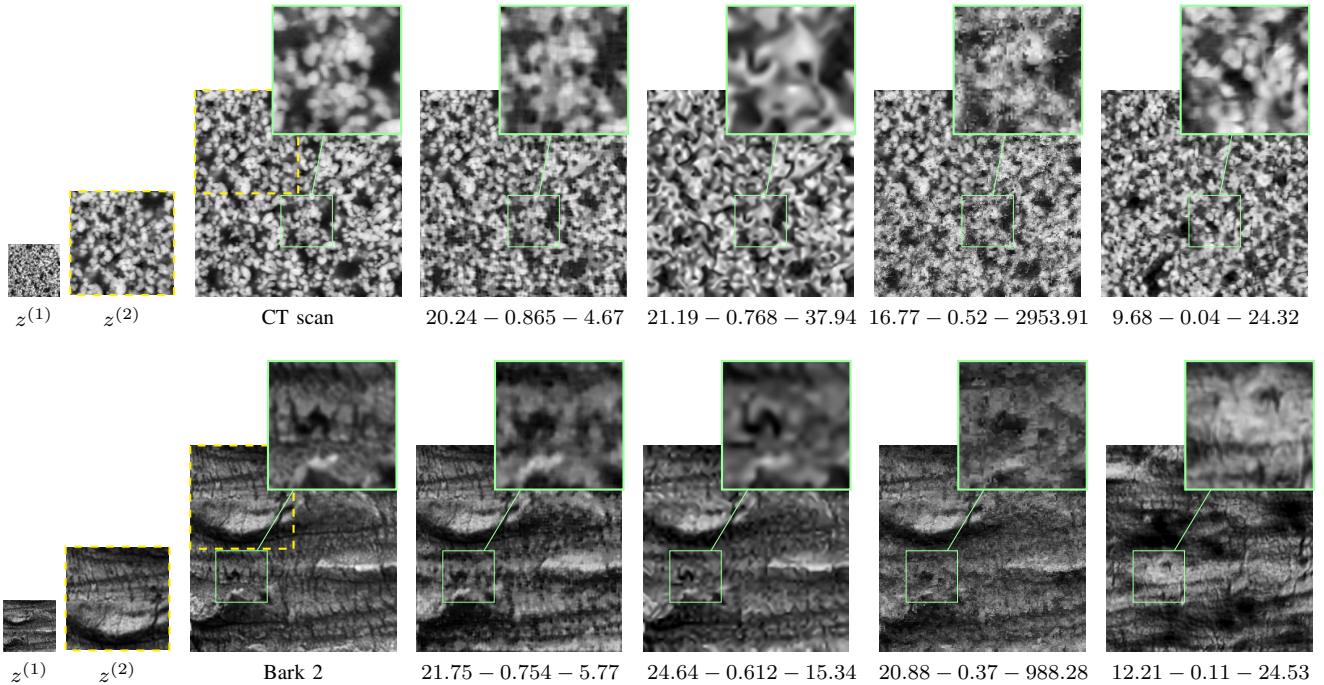
Fig. 7. PSNR – SSIM – \text{Err}_{\bar{x}} . From the left to the right: low-resolution image (down-sampling factor r = 4 , noise standard deviation \tau = 10 , blur 3 \times 3 ), high-resolution patch (25% of the total image), true image, proposed approach, Dong et al. [64], Hertzmann et al. [34] and Portilla et al. [65].
