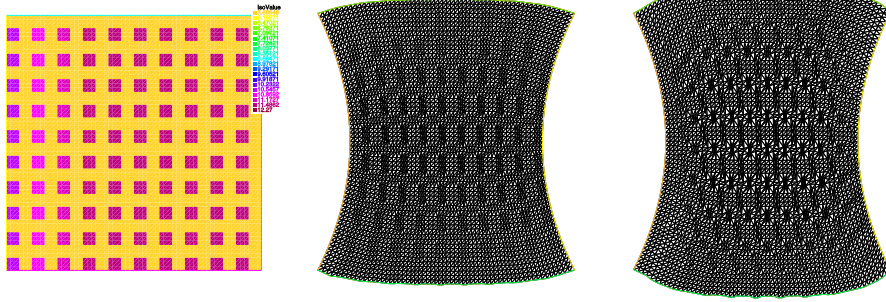
Fig. 1 Test case setup (all three configurations are drawn to scale). Left: Young's modulus – E = 10^6 with square inclusions of larger E , up to 10^{12} . Middle: Solution for \nu = 0.4 . Right: Solution for \nu = 0.49999 .
