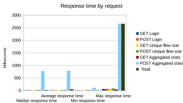
Figure 8. Statistics manager response time
