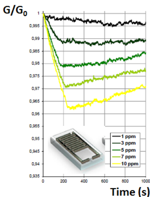
Figure 2. Conductimetric response to ammonia changes of a polypyrrole film deposited at +1 V/SCE from an aqueous electrolyte containing 0.1 M LiClO 4 .
