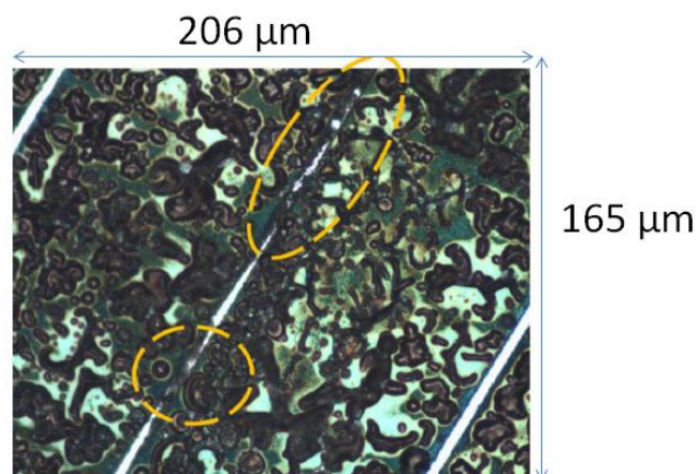
Figure 1. Optical microscopy picture of a polypyrrole film electrodeposited on platinum microelectrode arrays (gap between the arrays: 5 \mu\text{m} ).
