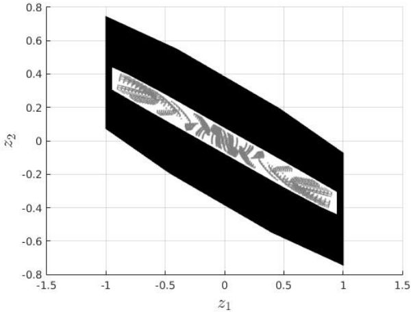
Figure 2: Sampled points of \Phi(S) (in grey), over-approximation \bar{\Phi}(S) given by Theorem 3 and over-approximation of (11) computed using Theorem 2 (in black).
