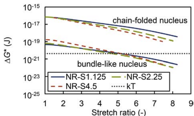
Fig. 8. Comparison of \Delta G^* with respect to the stretch ratio calculated with values of \sigma^2\sigma_e for folded-chain and bundle-like nuclei.
