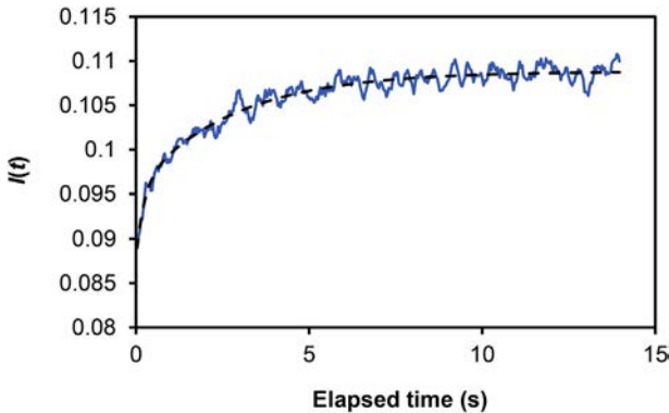
Fig. 2. Time-dependent change of experimental I(t) (solid line) and its regression curve (broken line). Sample: NR-S1.125, stretch ratio: 6, temperature: 29 °C.
