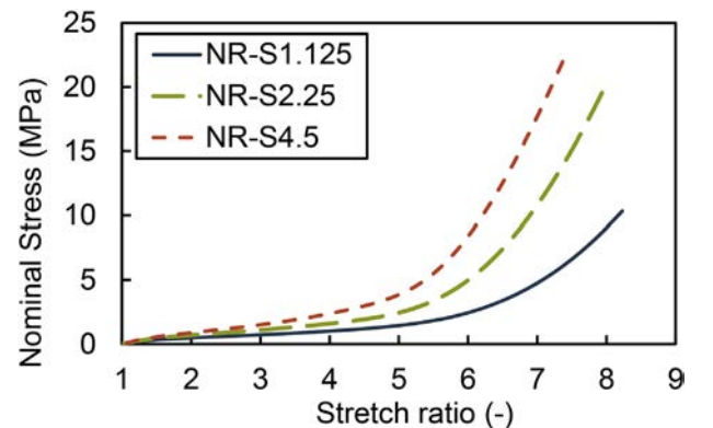
Fig. 4. Stress-strain curves of NR samples at 302 K.
