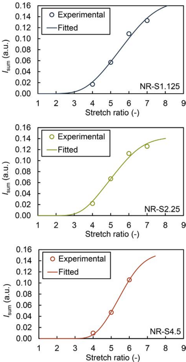
Fig. 7. Dependence of nucleation rate on stretch ratio at 302 K for bundle-like nuclei: experimental data (unfilled symbols) and fitted theoretical data (lines) with adjusted I_0 and \sigma^2\sigma_e .
