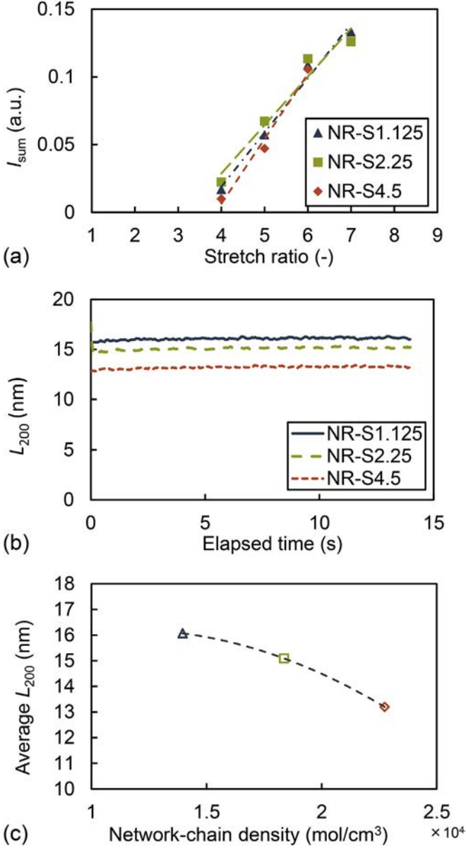
Fig. 3. Results of time-resolved WAXD measurements. (a) Dependence of the total increment of crystallinity index, I_{sum} , on stretch ratio. (b) Time evolution of crystallite size, L_{200} . (c) Dependence of crystallite size on network-chain density.
