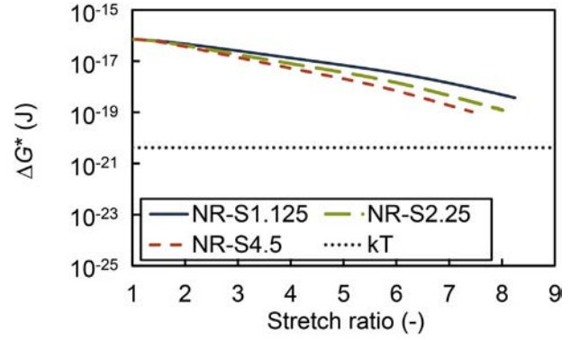
Fig. 6. Semilogarithmic scale plot of calculated \Delta G^* for a chain-folded nucleus as a function of stretch ratio at 302 K.
