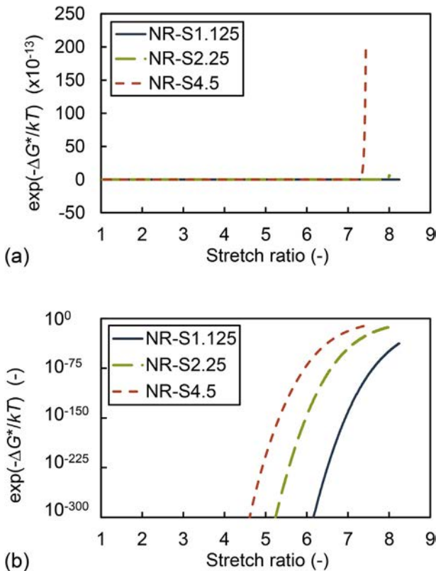
Fig. 5. Calculated dependence of I_{\text{sunv}}/I_0 = \exp(-\Delta G^*/kT) on stretch ratio \alpha at 302 K for chain-folded nuclei in linear scale (a) and semilogarithmic scale (b).
