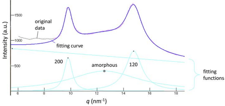
Fig. 1. An example of decomposition of WAXD intensity distribution. A part ( q < 9 \text{ nm}^{-1} ) of the original data (dotted line) was excluded from the fitting Sample: NR-S1.125, stretch ratio: 6, temperature: 29 °C, t :14 s.
