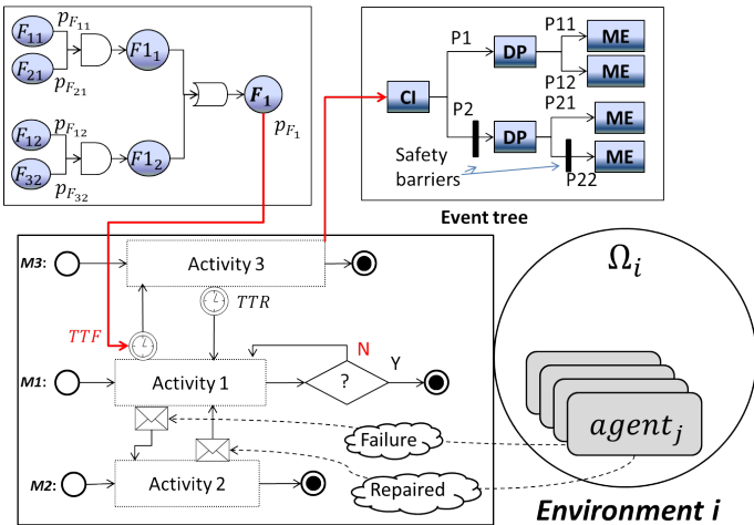
Fig. 3. Generic Agent-oriented risk model (agent i)
