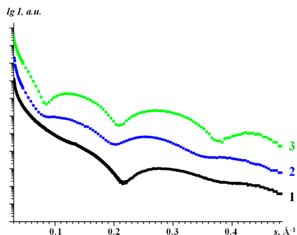
Figure 5. X ray reflectivity curves of CrHCR LB films transferred onto silicon substrate from pure water subphase at surface pressure π of 8 mN/m (1) and 25 mN/m (2) and transferred from the surface of a Ba(ClO 4 ) 2 aqueous solution (1 mM) at π = 25 mN/m (3).
