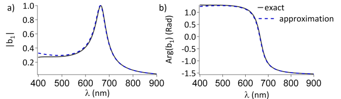
FIG. 2: Approximate values for the magnetic dipole Mie coefficient, b_1 , (amplitude and phase - dashed blue), compared with the exact values (solid black); R = 80 nm, \epsilon = 16 .
