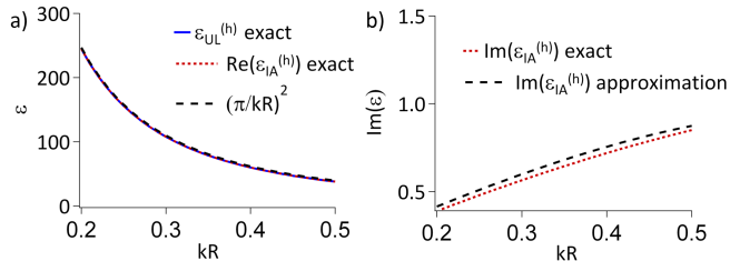
FIG. 7: Permittivities satisfying the magnetic dipole UL, \varepsilon_{\text{UL}}^{(h)} , [solid (blue) line] and satisfying magnetic IA, \varepsilon_{\text{IA}}^{(h)} [dotted (red) line] as functions of kR : real parts (a) and imaginary parts (b). Approximate algebraic expressions of Eqs.(15) and (16) are plotted by the dashed black line.
