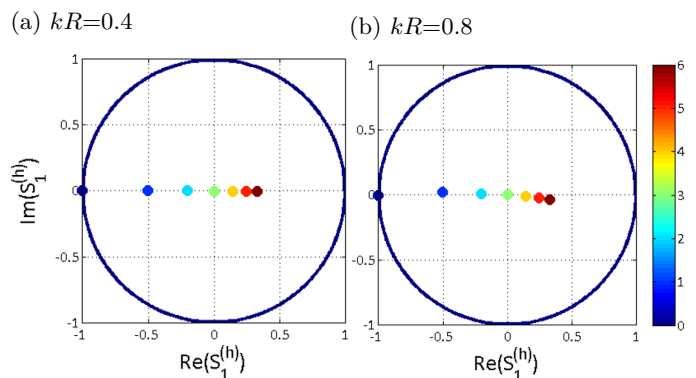
FIG. 8: Values of S_1^{(h)} for permittivities calculated from Eq.(17) for kR = 0.4 and kR = 0.8 ; the color bar indicates the value of j at each point.
