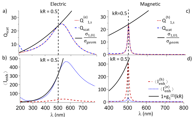
FIG. 5: Cross section efficiencies (a,c) and field enhancements at the particle surface (b,d) for R = 40 -nm spheres satisfying the dipole UL in the electric (a,b) and magnetic (c,d) modes at kR = 0.5 . Maximal dipole contributions to Q and \langle I_{\text{enh}}^{(e,h)} \rangle are plotted as solid black lines.
