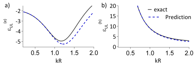
FIG. 3: Values of permittivity required to reach the dipole UL in the electric (a) and magnetic (b) modes as a function of kR . Exact predictions (black lines) and approximate predictions (dashed (blue) lines).
