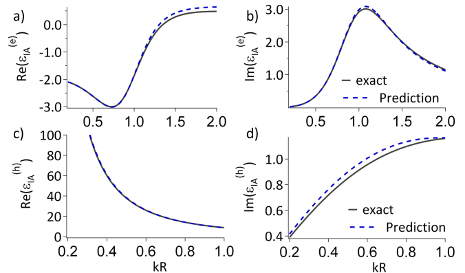
FIG. 4: Real (a,c) and imaginary (b,d) parts of the dielectric permittivity satisfying IA in the electric (a,b) and magnetic (c,d) dipole modes. Exact predictions (full black lines) and approximate predictions (dashed (blue) lines).
