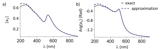
FIG. 1: Approximate values for the electric dipole Mie coefficient, a_1 , (amplitude and phase - dashed blue), compared with the exact values (solid black); R = 60 -nm gold sphere.
