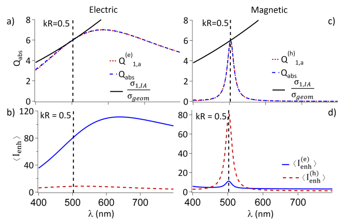
FIG. 6: (Colour online) The same plots as in Fig.5 except that absorption efficiencies in dipole IA particles in (a) and (c) are plotted at kR = 0.5 . Dipole absorption limit efficiencies are plotted by solid black lines.
