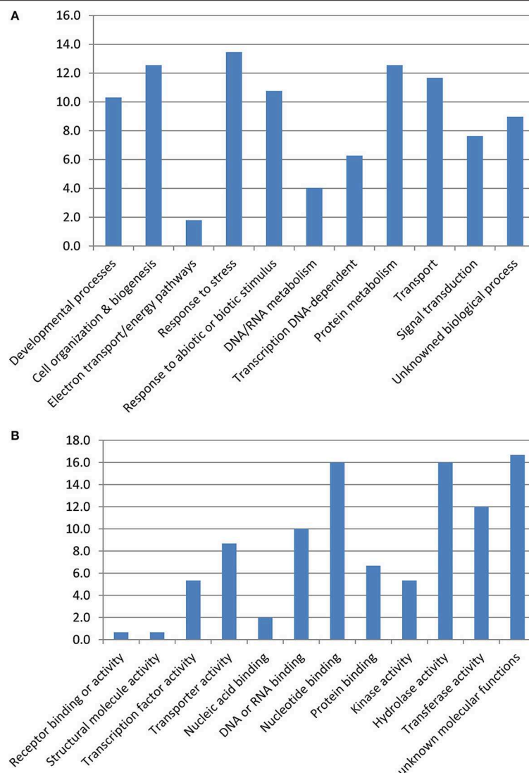
FIGURE 2 | Gene ontology terms associated to SNP/genes associated to resistance to stem canker. Gene ontology terms for biological process (A) and molecular activity (B).
