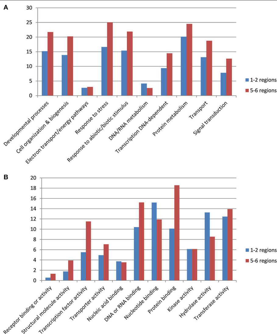
FIGURE 1 | Gene ontology terms associated to genes retained in 1–2 or 5–6 duplicated regions. Gene ontology terms for biological process (A) and molecular activity (B).
