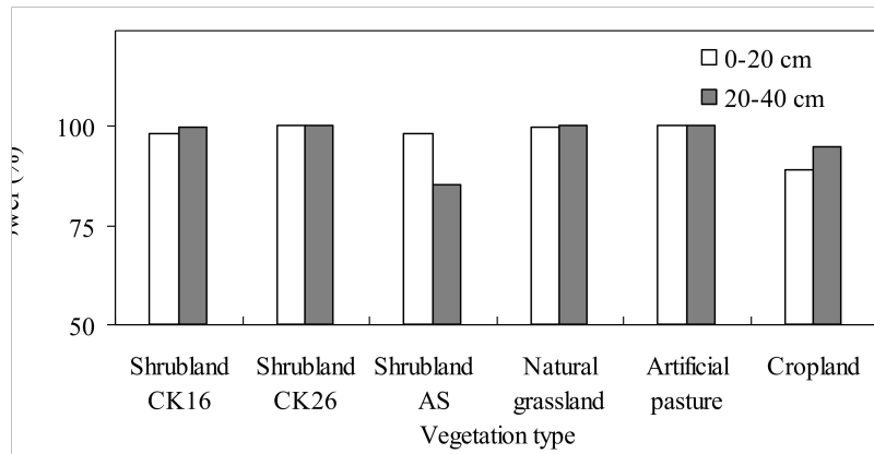
Fig. 2. Probability (power) of detecting a 25 % uncertainty in soil organic carbon stocks with a 0.05 level of significance for vegetation types at 0-20 and 20-40 cm soil layers.
