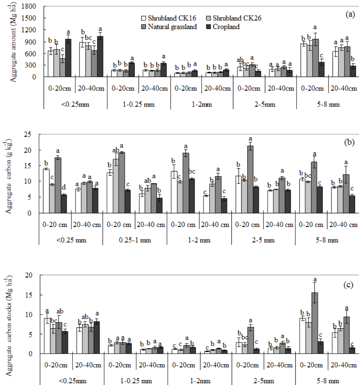
Fig. 3. Vegetation types and (a) aggregate amount, (b) soil organic carbon concentration in aggregate fractions, (c) soil organic carbon stocks in aggregate fractions.
