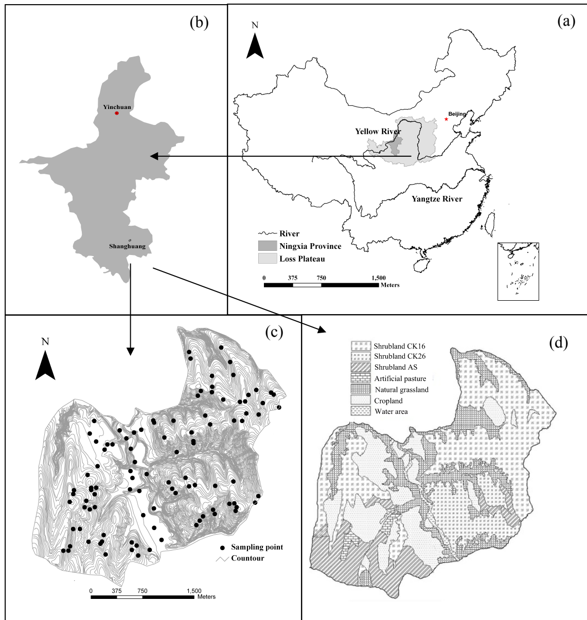
Fig. 1. The location of the study area and its land use. (a) Location of the Ningxia Province and the Loess Plateau in China; (b) Location of the Shanghuang study area in the Ningxia Autonomous Region, (c) Contour lines and soil sampling sites in the study area, (d) Vegetation types of the study area.
