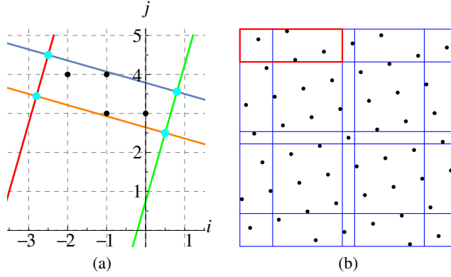
Fig. 5: (a) Geometrical interpretation of the system of linear inequalities in Equation (7), in the (i, j) -plane for (p, q) = (7, 2) . The region surrounded by the four lines is \hat{f}_{\downarrow}^2 , and the integer points within are marked by black circles. (b) The remainder range, C_{\downarrow}^{\sigma} and f_{\downarrow}^2 illustrated by a red square, which corresponds to \hat{f}_{\downarrow}^2 in (a).
