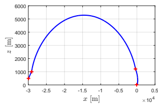
Fig. 16. Optimal trajectory in ( x, z ) plane.
