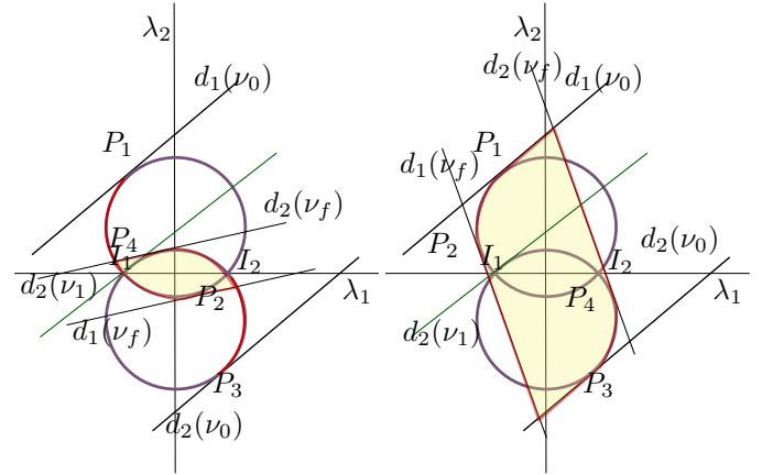
Fig. 2. Feasible set defined by two circle arcs and two segments (case IIa).
