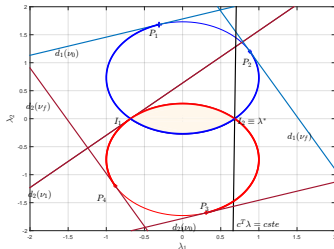
Fig. 8. Feasible set and optimal solution for GTO mission example.
