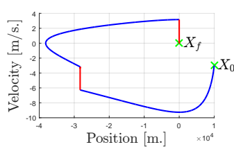
Fig. 7. Optimal trajectory in phase plane.
