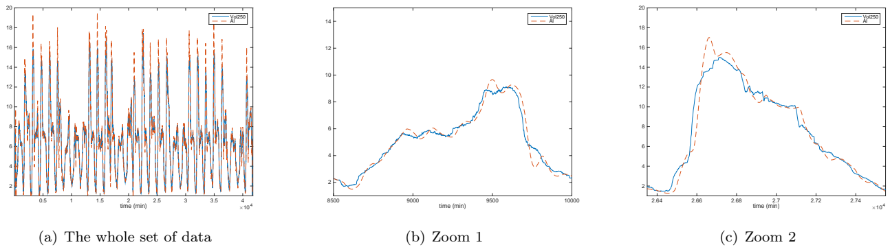
Fig. 8. Forecasting volatility
