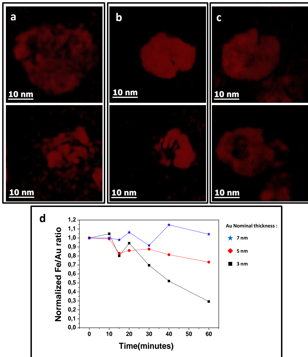
Figure 6: Degradation of iron oxide NFs as a function of the nominal thickness of the protective gold layer. Bragg filtered high resolution images showing only the iron oxide NFs before (top image) and after 45 minutes in the lysosome-like medium (bottom image). The nominal thickness of the gold layer is (a) 3 nm (isolated clusters), (b) 5 nm (percolated film) and (c) 7 nm (continuous layer). (d) EDX quantitative measurement of the Fe/Au ratio in single Au-coated
