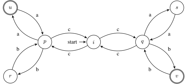
Figure 7: Automaton \mathcal{B}_2
