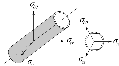
FIGURE 4 – von Mises and Tresca yield surfaces
