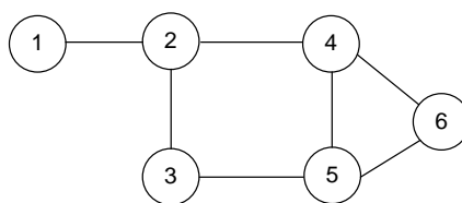
Figure 2. A disjunctive graph
