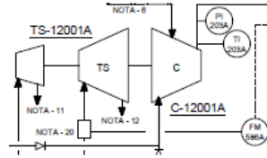
Fig. 1. P&ID of a compressor unit of the gas compression station.
