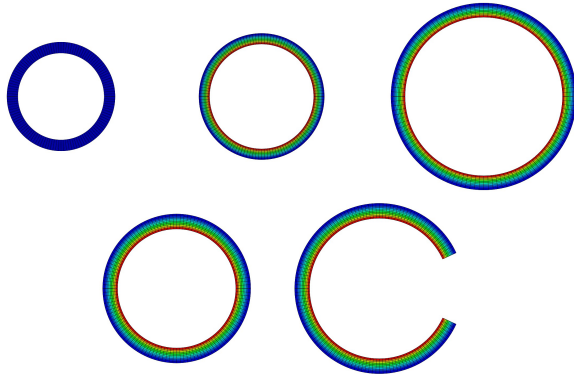
Figure 3. Growth-induced residual stresses and virtual opening angle experiment on an artery.
