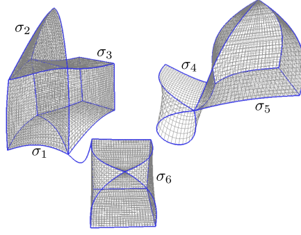
Figure 9: A simplicial Bézier space of dimension 3. Note that \sigma_1 is a prism (i.e. simploid of type (2, 1) ) connecting the simplex \sigma_2 and the cube \sigma_3 , \sigma_4 is a square (i.e. simploid of type (1, 1) ) such that one of its edge is a self loop, \sigma_6 is a cube (i.e. simploid of type (1, 1, 1) ) with a degenerate edge, and \sigma_5 is a cone over a square face (i.e. a simploid of type (1, 1, 1) with a degenerate face).
