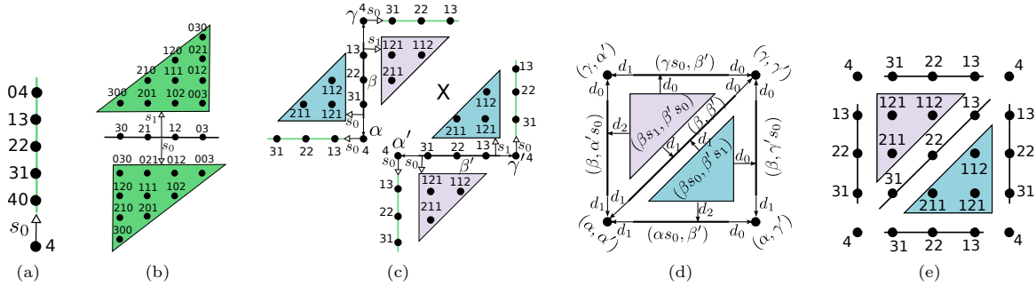
Figure 8: (a) According to Property 1, if all the control points of the degenerate edge are equal to the vertex, then the Bézier simplex corresponding to the edge is equal to the Bézier simplex corresponding to the vertex. (b) illustrates an edge and its two possible degenerate triangles. According to Property 1, if all control points (of a triangle) which are aligned vertically are equal to the control point on the edge in the same alignment, then the Bézier triangles and the Bézier edge are equal. (c) Cartesian product of two edges: the useful degenerate simplices are represented up to dimension 2. According to Property 1, all proper control points of the degenerate edge \alpha s_0 (resp. \gamma s_0 ) are equal to control point P_4 of vertex \alpha (resp. \gamma ); and proper control points P_{211} and P_{121} (resp. P_{112} ) of the degenerate edge \beta s_0 are equal to control point P_{31} (resp. P_{22} ) of \beta . Similarly, proper control points P_{121} and P_{112} (resp. P_{211} ) of degenerate simplex \beta s_1 are equal to control point P_{13} (resp. P_{22} ) of \beta . (d) the simplicial set resulting from the cartesian product of the two edges of (c). Each 2–simplex in (d) is the simplex resulting from the cartesian product of the two 2–simplices of the same color in (c). For example, \beta s_0 \times \beta' s_1 is the simplex (\beta s_0, \beta' s_1) . For clarity purpose, the control points are displayed in (e).
