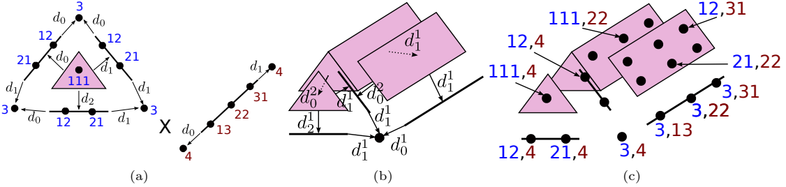
Figure 6: a) and b): correspondence between the product of two simplices (and their boundaries) and a simploid of type (2, 1) . For clarity purpose, only a part of its boundary is displayed and some of its control points are displayed in c).
