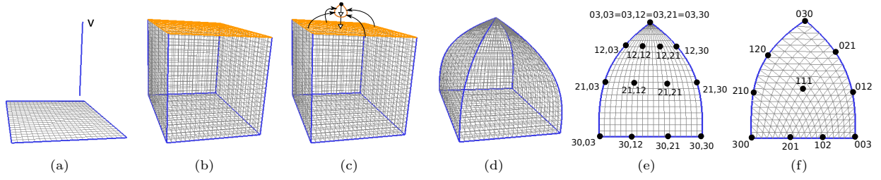
Figure 10: (a) The cone applied to a square (and its boundary) is a square-based pyramid (d). Thanks to degeneracy operators, the cone operation consists in an extrusion (a) – (b) followed by the degeneracy of the copy of the original simploidal set (in orange in (b)). In practice, the computation can be improved by creating directly all the degenerate simploids incident to the new vertex and then setting all the boundary and degeneracy operators (c). (e) the structure of the control points of a lateral Bézier square face of (d) is different from the structure of the control points of a Bézier triangle (f).
