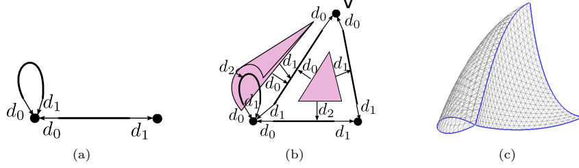
Figure 4: The semi-simplicial set b ) can be obtained by a cone operation applied to the semi-simplicial set of a ), v is the new vertex. c ) is a geometric representation of semi-simplicial set b ).
