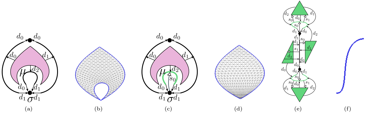
Figure 7: (a) a semi-simplicial set and (b) its associated Bézier triangular space. (c) a simplicial set: the green edge \mu is degenerate into the bottom vertex \sigma . Otherwise said, \mu = \sigma s_0 . (d) the corresponding triangular Bézier space: the degenerate edge is reduced to a point, corresponding to its incident vertex. Note that edge \mu is the only degenerate simplex which is a face of a non degenerate one. (e) a simplicial set representing an edge (and its boundary) and all its degenerate simplices up to dimension 2 (in green) and (f) its corresponding Bézier triangular space.
