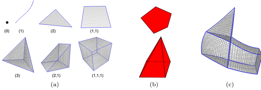
Figure 1: (a) Simploids and their types. (b) Counterexamples of simploids: a pentagon and a pyramid (i.e. a cone on a square face): the main cells are not the cartesian product of simplices. (c) A geometric representation of a simploidal set made of 3–dimensional simploids: a tetrahedron (type (3)), a cube (type (1, 1, 1)) and a prism (type (2, 1) or (1, 2)).
