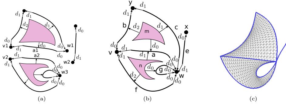
Figure 2: (a) A semi-simplicial set. Semi-simplicial set (b) is obtained by identifying vertices v_1 and v_2 , vertices w_1, w_2 and w_3 , and edges a_1 and a_2 . (c) A geometric representation of semi-simplicial set (b). The commutation properties satisfied by face operators guarantee the consistency of the data structure. For example, for any triangle \sigma : \sigma d_2 d_1 = \sigma d_1 d_1 , \sigma d_2 d_0 = \sigma d_0 d_1 , and \sigma d_1 d_0 = \sigma d_0 d_0 , so a triangle has at most 3 vertices in its boundary.
