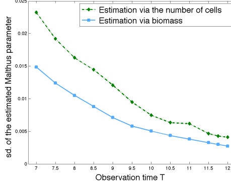
FIGURE 3. Model (S+V). Standard deviation of two estimators of the Malthus parameter as T increases (based on M = 50 Monte Carlo continuous time trees simulated up to time T ), for \rho_{\alpha=0.3} and division rate \gamma(x, v) = vxB(x) with B(x) = (x - 1)^2 \mathbf{1}_{\{x \geq 1\}} . Blue lower curve: estimation by (16) via the biomass. Green upper curve: estimation by (33) via the number of cells.
