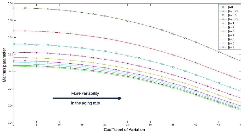
FIGURE 1. Model (A+V). CV_{\rho_\alpha} \rightsquigarrow \lambda_{B,\rho_\alpha} defined by (11) for \rho_\alpha(v) = \alpha^{-1}\rho(\alpha^{-1}(v - (1 - \alpha)\bar{v})) (the baseline density \rho is a Gaussian density with mean \bar{v} = 1 and standard deviation 0.7 truncated on [0, 2] ) and different division rates \gamma(a, v) = vB(a) with B(a) = (a - 1)^\beta \mathbf{1}_{\{a \geq 1\}} , \beta \in \{0, 0.25, 0.5, 0.75, 1, 2, \dots, 7\} . Reference (all cells age at rate \bar{v} = 1 ): point of null abscissa and y-coordinate \lambda_{B,\bar{v}=1} defined by (10).
