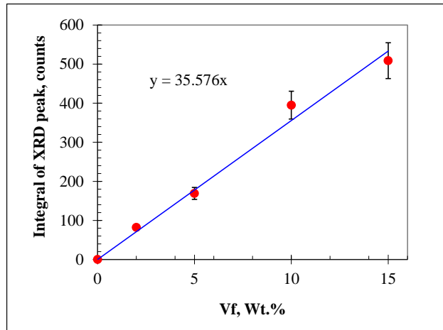
Fig. 4. Calibration curve for the volume fraction of NaF crystals measured by mixing virgin PTR glass powder with known volume fraction of pure NaF crystals powder and measuring the X-ray diffraction pattern.
