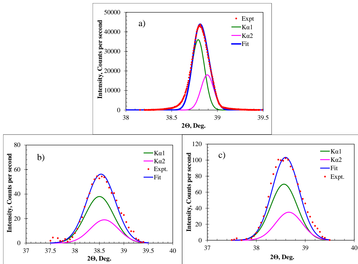
Fig. 2. Modeling of the X-ray diffraction peak of NaF crystals measured in a) pure NaF crystal powder b) PTR glass exposed to 0.9 \text{ J/cm}^2 at 325 nm, pre-nucleated for 100 minutes at 485^\circ\text{C} and thermally developed for 2 hours at 515^\circ\text{C} c) similar PTR glass as b) but thermally developed for 6 hours at 515^\circ\text{C} .
