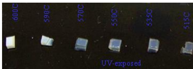
Fig. 9. Pictures of PTR glass samples exposed to 0.9 \text{ J/cm}^2 at 325 nm, pre-nucleated for 100 minutes at 485^\circ\text{C} and isothermally treated in DSC at different temperature until reaching overall crystallization.
