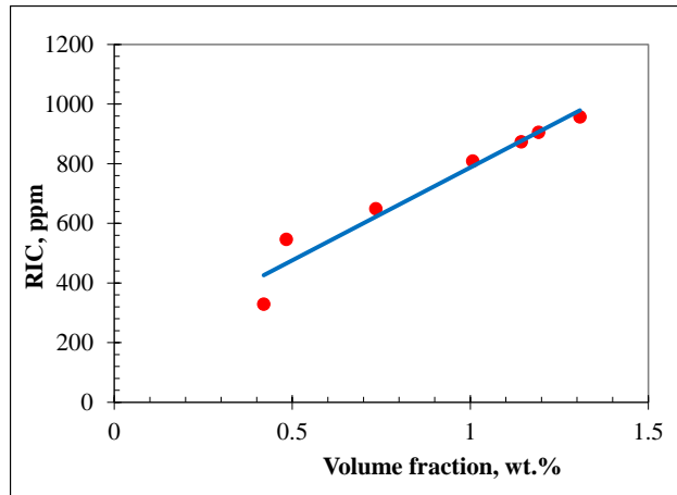
Fig. 8. Evolution of the refractive index change measured in PTR glass exposed to 0.9 \text{ J/cm}^2 at 325 nm, pre-nucleated for 100 minutes at 485^\circ\text{C} and thermally developed at 515^\circ\text{C} for different durations as a function of the NaF crystals volume fraction.
