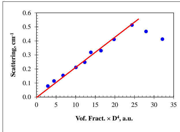
Fig. 7. Evolution of the scattering at 633 nm measured in PTR glass exposed to 0.9 \text{ J/cm}^2 at 325 nm, pre-nucleated for 100 minutes at 485^\circ\text{C} and thermally developed at 515^\circ\text{C} for different durations (Blue dots) as a function of the product between the NaF crystals volume fraction and the fourth power of the crystal radius, and its fit using a linear function (red line).
