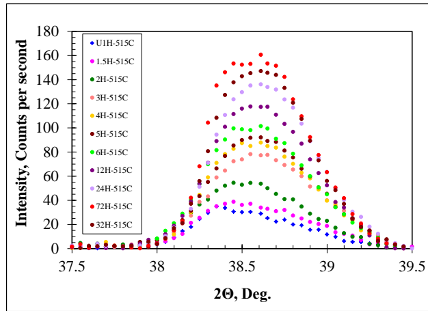
Fig. 1. Evolution of the X-ray diffraction peak of NaF crystals measured in PTR glass exposed to 0.9 \text{ J/cm}^2 at 325 nm, pre-nucleated for 100 minutes at 485^\circ\text{C} and thermally developed at 515^\circ\text{C} for different durations.
