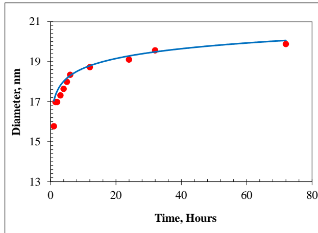
Fig. 6. Evolution of the average NaF crystal diameter extracted from the NaF X-ray diffraction peak measured in PTR glass exposed to 0.9 \text{ J/cm}^2 at 325 nm, pre-nucleated for 100 minutes at 485^\circ\text{C} and thermally developed at 515^\circ\text{C} for different durations.
