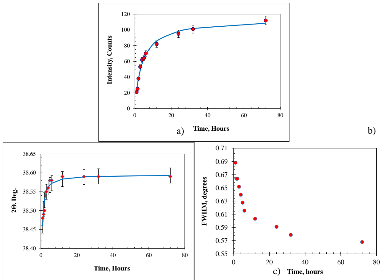
Fig. 3. Evolution of the parameters (peak intensity (a), position (b) and FWHM (c)) extracted from the X-ray diffraction peak of NaF crystals measured in PTR glass exposed to 0.9 \text{ J/cm}^2 at 325 nm, pre-nucleated for 100 minutes at 485^\circ\text{C} and thermally developed at 515^\circ\text{C} for different durations.
