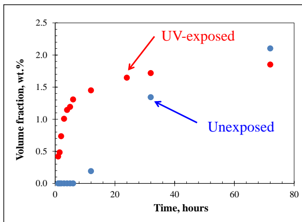
Fig. 5. Evolution of the volume fraction of NaF crystals measured in PTR glass exposed to 0.9 \text{ J/cm}^2 at 325 nm, pre-nucleated for 100 minutes at 485^\circ\text{C} and thermally developed at 515^\circ\text{C} for different durations (Red curve). For reference the evolution of the volume fraction of NaF crystals measured in unexposed PTR glass thermally treated in the same condition is shown (Blue curve).
