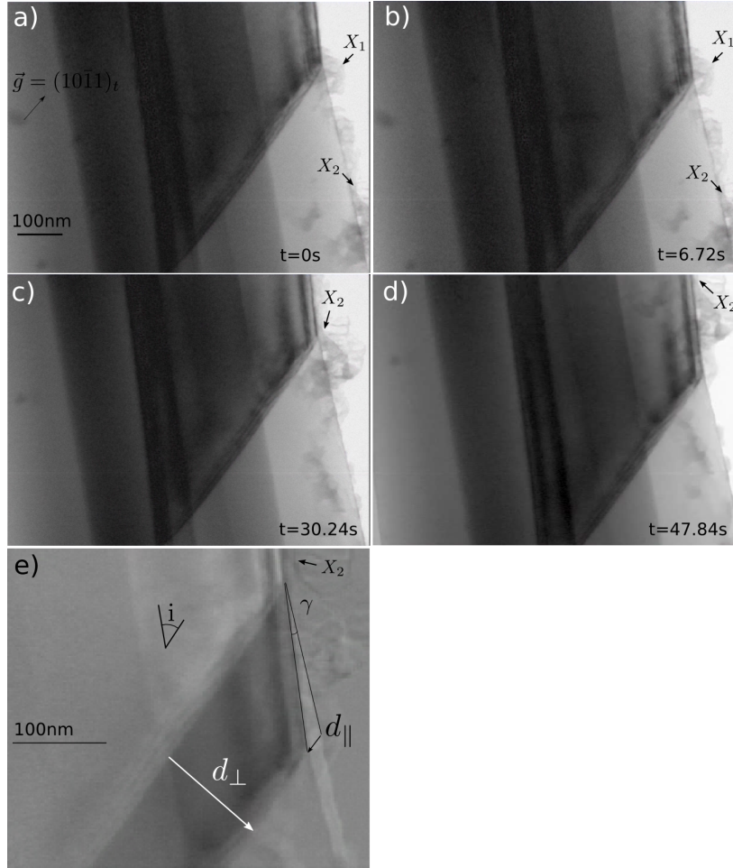
Figure 3: a) to d) show the migration of a (01\bar{1}2) twin boundary under stress. X_1 and X_2 are fiducial markers. e) is the image difference d-c when X_2 position is set as a reference. This allows the measure of both the migration distance ( d_{\perp} ) and the shear displacement ( d_{\parallel} ).
