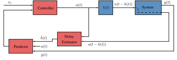
Fig. 5. Closed-loop scheme with the combination of the delay estimator and the predictor (see Remark 2 for the dashed line)
