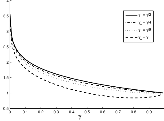
Figure 1: Function \sqrt{z_{\gamma_+} \varphi(z_{\gamma_+})/\gamma - z_{1-\gamma_-} \varphi(z_{1-\gamma_-})/\gamma} + 1 as a function of the percentage \gamma of individuals genotyped and as a function of the ratio \gamma_+/\gamma .
