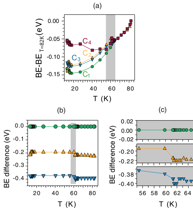
FIG. 13. (Color online) Critical behavior extracted from CL deconvolution analysis. (a) BEs (referred to their value at 82 K) vs temperature. (b) Closer view of the BE evolution measured with respect to C_1 (green circles), which removes the SPV shift of C_2 (yellow up triangles) and C_3 (blue down triangles). (c) Closer view of the critical temperature range around 60 K highlighted with a gray shadowing in all the panels (values for C_1 – C_3 are represented by the same markers and colors as in previous panels).
