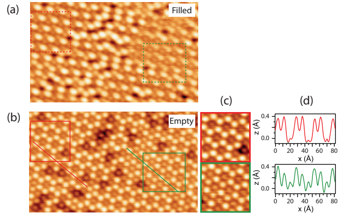
FIG. 5. (Color online) Complementary STM images ( 17 \times 10 \text{ nm}^2 ) of the same region obtained sequentially (a) for filled ( V = -1.0 \text{ V} ; I = 1.0 \text{ nA} ) and (b) for empty ( V = +1.0 \text{ V} ; I = 1.0 \text{ nA} ) states. As there is a significant number of defects, we observe coexistence of metallic- (3 \times 3) (red squares) and COI- (3 \times 3) (green squares). Panel (c) shows a zoom ( 4 \times 4 \text{ nm}^2 ) of both empty states square areas from panel (b). Using empty states images, both phases can only be distinguished from an analysis of the height profiles, as shown in panel (d) for profiles along the two lines appearing in panel (b).
