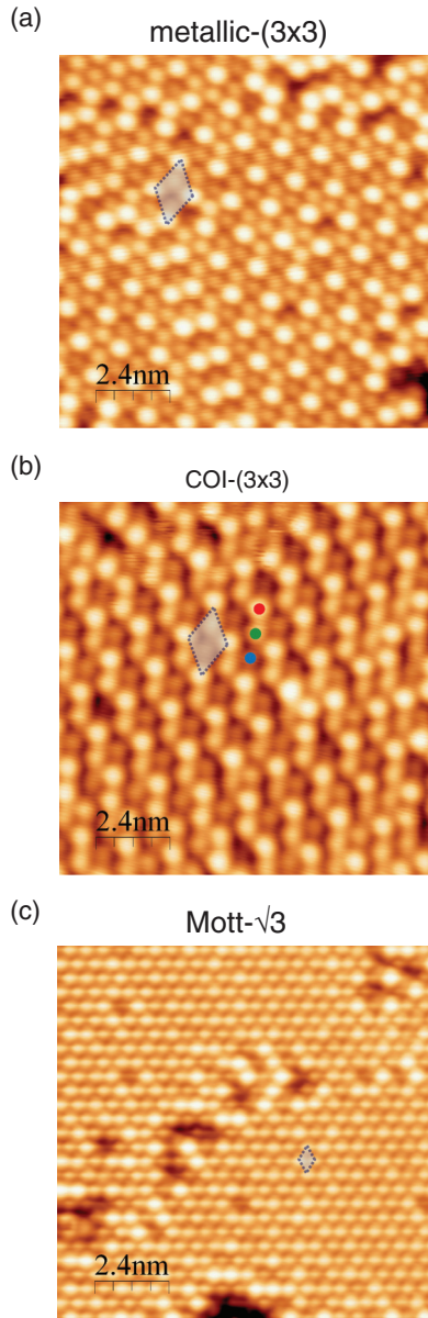
FIG. 4. (Color online) (a) Metallic-( 3 \times 3 ) phase ( 12 \times 12 \text{ nm}^2 ; V = -1.0 \text{ V} ; I = 0.525 \text{ nA} ; T = 78 \text{ K} ). (b) COI-( 3 \times 3 ) structure ( 12 \times 12 \text{ nm}^2 ; V = -1.0 \text{ V} ; I = 1.0 \text{ nA} ; T = 60 \text{ K} ). Dots mark up (red), middle (green), and down (blue) atoms. (c) Mott- \sqrt{3} phase ( 12 \times 12 \text{ nm}^2 ; V = -1.4 \text{ V} ; I = 1.0 \text{ nA} ; T = 5 \text{ K} ). In every panel, a unit cell of the corresponding phase is highlighted.
