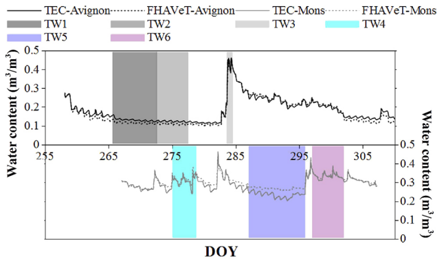
Figure 5. Soil water content evolution in time for the 0–5 cm layer; comparison between models – soil AL-SiL, PTF – Wosten. Avignon climate (top) and Mons climate (bottom).
