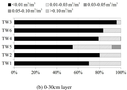
Figure 6. Absolute water content difference distribution between the developed model and TEC for each climatic case study.
