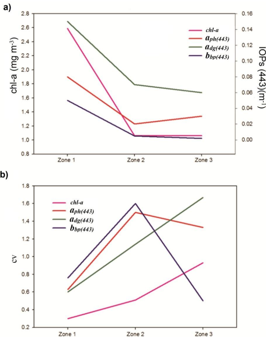
Figure 4. Climatology of the IOPs in the study area. (a) Mean values; (b) coefficient of variation.
