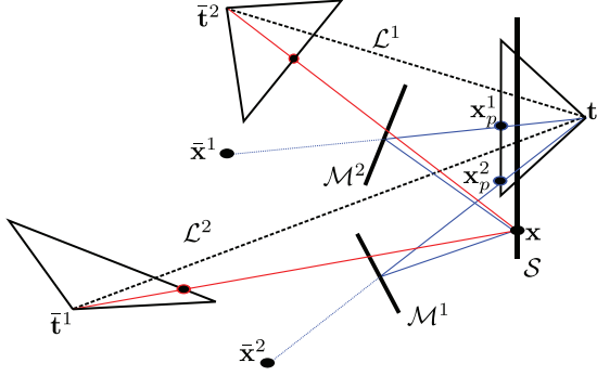
Fig. 10. 2D-representation of the geometric model. A point x on the screen S is reflected by the mirror \mathcal{M}^i , i=1,2 , and projected on the pixel x_p^i of the real camera (blue line), as if the camera was directly observing the mirrored point \bar{x}^i . On the other hand, the reflection by the mirror \mathcal{M}^i defines a mirrored (virtual) camera which directly observes the real point x (red line).
