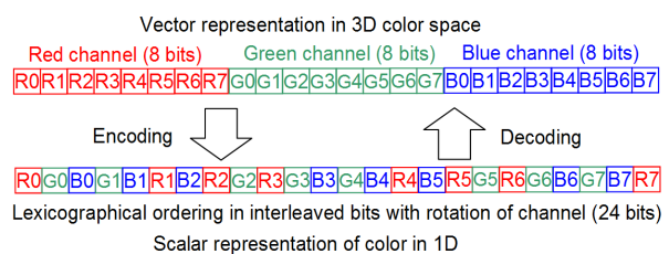
Figure 2: Color coding in scalar by using interleaved bit and rotation of the sequence of RGB.
