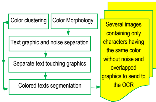
Figure 3: illustrates the overall scheme of ACoDPS.
