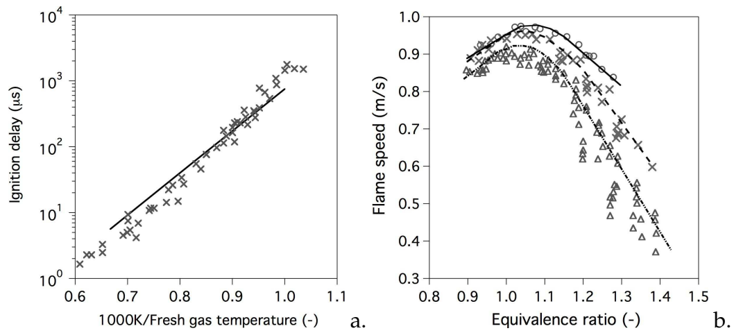
Fig. 1. a) Ignition delay versus inverse of fresh gas temperature: experimental data provided in [41–43] ( \times ) and results of Eq. (1) (—); b) Laminar flame speed versus equivalence ratio at P = 1 \text{ atm} and fresh gas temperature T_f = 473 \text{ K} for kerosene ( \Delta ), n-decane ( \circ ) and a mixture of n-decane/n-probylbenzene ( \times ) [39].
