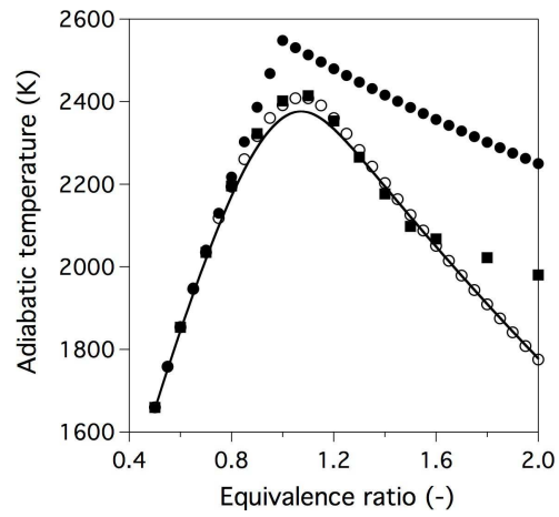
Fig. 6. Adiabatic temperature versus equivalence ratio at fresh gas temperature T_f = 473\text{ K} and pressure P = 1\text{ atm} . Comparison between the LUCHE skeletal mechanism [40] (—) and simplified mixtures composed of 5 (●), 6 (■) and 7 (○) species (Equilibrium computations with CANTERA).
