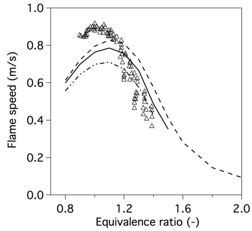
Fig. 2. Flame speed versus equivalence ratio at fresh gas temperature T_f = 473\text{ K} and pressure P = 1\text{ atm} . Comparison between the DAGAUT detailed mechanism [41] (---), the EL-BAKALI_RISTORI detailed mechanism [57] (—), the LUCHE skeletal mechanism [40] (— · —), and the experimental results [39] ( \Delta ).
