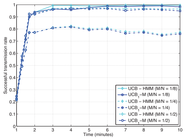
Fig. 8. Successful transmission rate of hybrid UCB-HMM system and UCB_1 - M with \alpha = 0.4 and M/N = \{1/8, 1/4, 1/2\} .
