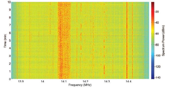
Fig. 2. Example of a measurement of the High Activity scenario (acquired at weekends) of the HF database [4].
