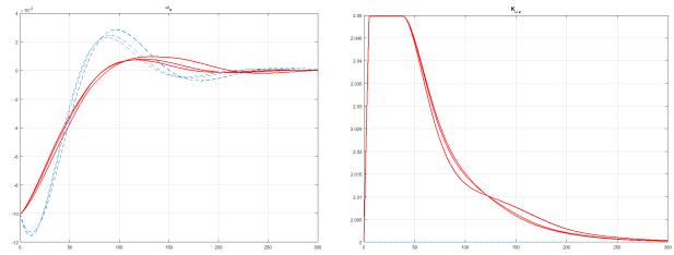
Figure 6: z-axis. Left: Angular rate; Right: Gain K_{\omega z} . Dashed: without adaptation. Solid: with adaptation
