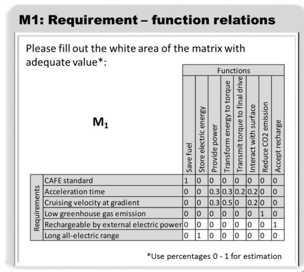
Fig. 11 Requirement – function relations
