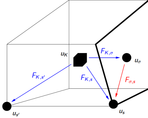
Figure 3: Matrix fluxes (in blue) and fracture fluxes (in red) inside a cell K with a fracture face \sigma (in bold). The matrix fluxes F_{K,\nu} connect the cell K to its nodes and fracture faces \nu \in \mathcal{V}_K \cup \mathcal{F}_{\Gamma,K} . The fracture fluxes F_{\sigma,\mathbf{s}} connect the face \sigma to the nodes \mathbf{s} \in \mathcal{V}_\sigma of \sigma .
