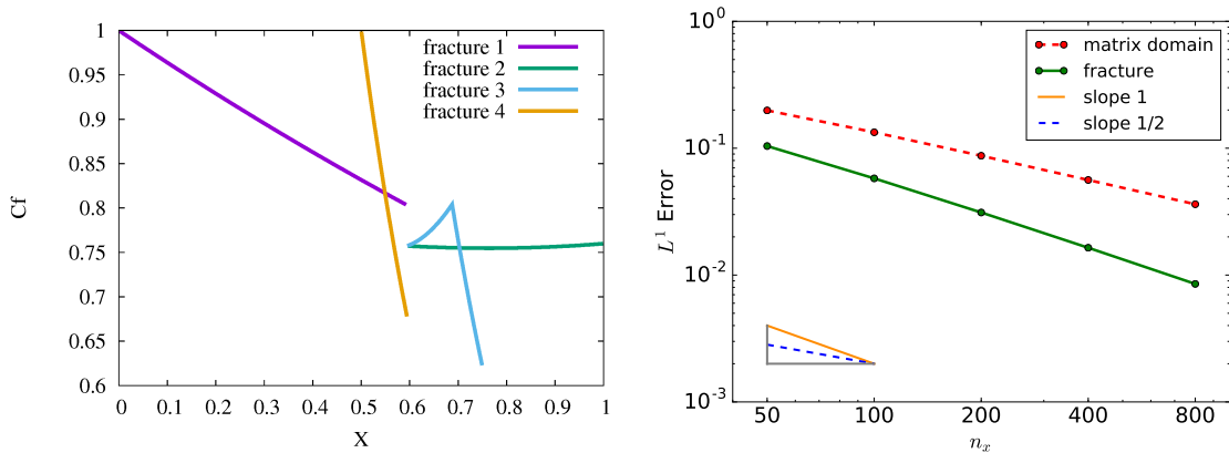
Figure 10: Left: stationary analytical solution in the four fractures as a function of the x coordinate. Right: relative L^1 errors and references in the matrix domain and in the fracture network between the stationary analytical and numerical solutions as a function of the grid size n_x = 100, 200, 400, 800 .
