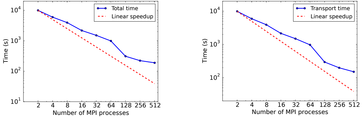
Figure 13: Total computation time (left) and computation time for the transport model (right) vs. the number of MPI processes for the mesh size n_x = 128 .
