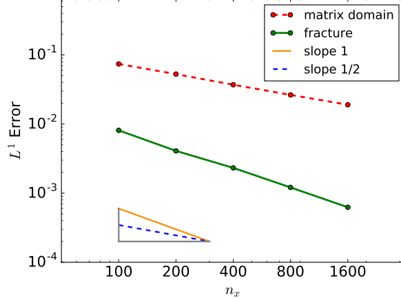
Figure 8: Relative L^1 errors and references in the matrix domain and in the fracture at time t_f between the analytical solution and the numerical solutions as a function of the grid size n_x = 100, 200, 400, 800, 1600 .
