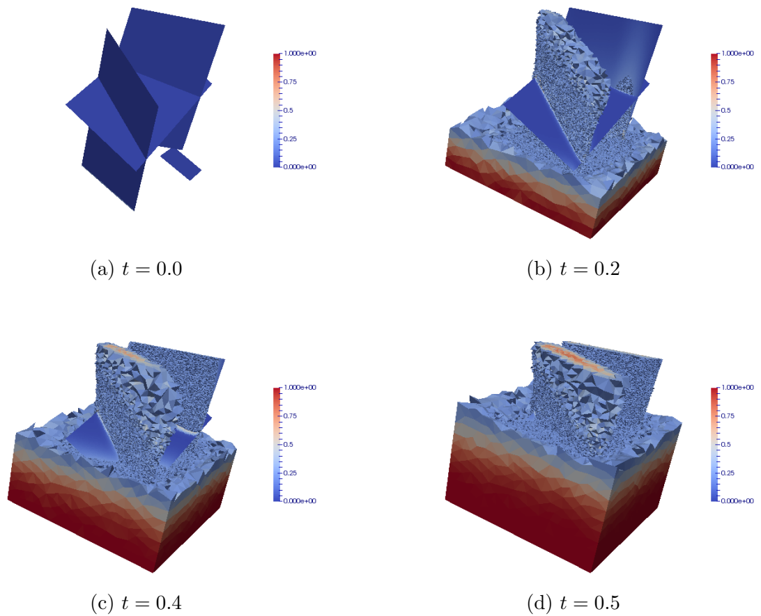
Figure 15: Concentration in the matrix domain and in the fracture network obtained at different times for the tetrahedral mesh. A threshold of 0.2 is used in the matrix domain.
