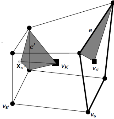
Figure 2: For a cell K with one fracture face \sigma in bold: cell unknown v_K located at \mathbf{x}_K , fracture-face unknown v_{\sigma} located at \mathbf{x}_{\sigma} , node unknowns v_{\mathbf{s}}, v_{\mathbf{s}'} , face centre \mathbf{x}_{\sigma'} of face \sigma' , triangle T_{\sigma,e} (convex hull of e and \mathbf{x}_{\sigma} ), triangle T_{\sigma',e'} (convex hull of e' and \mathbf{x}_{\sigma'} ) and tetrahedron T_{K,\sigma',e'} (convex hull of \mathbf{x}_K , \mathbf{x}_{\sigma'} and e' ).
