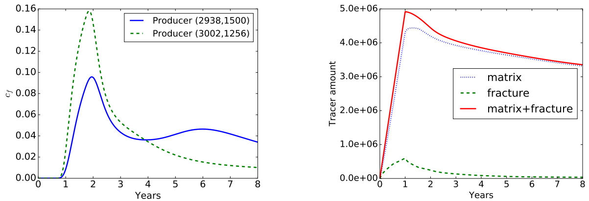
Figure 19: Mean tracer concentration in both production wells as a function of time (left) defined as the ratio between the well tracer flow rate and the well fluid flow rate (equal in our case to the well fracture-face tracer concentration). Volume of tracer as a function of time in the matrix domain, in the fracture network and their sum (right).
