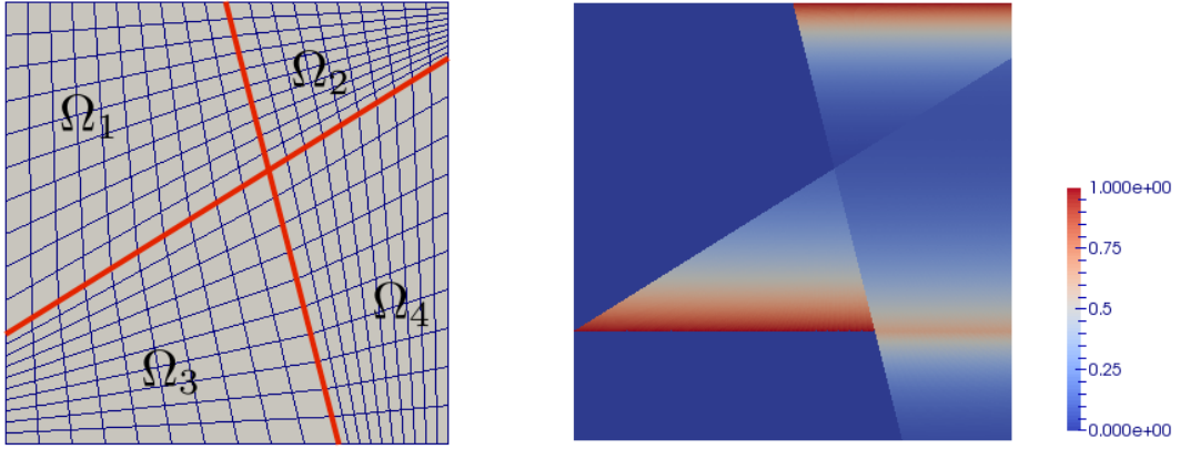
Figure 9: Left: example of mesh with n_x = 20 where the red lines account for the four fractures. Right: stationary analytical solution of (18).
