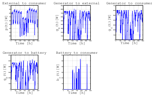
(c) Control inputs
