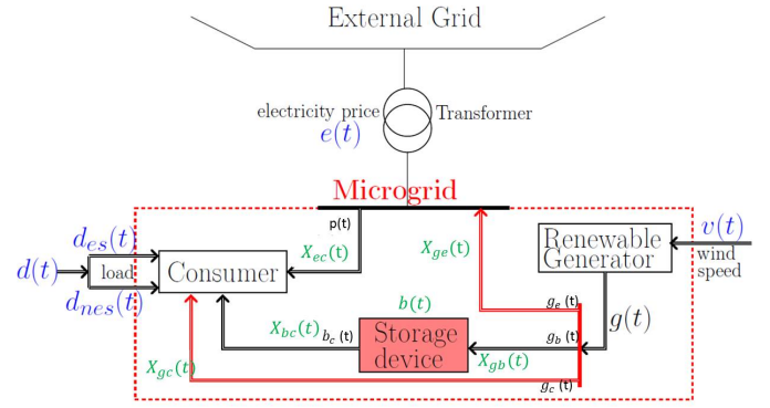
Figure 1: Microgrid
