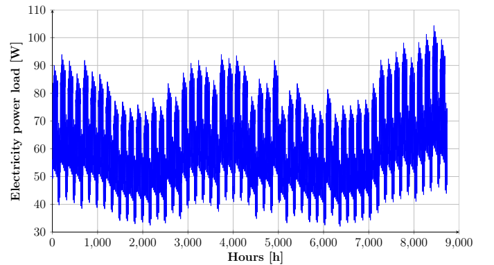
Figure 2: Consumer load profile
