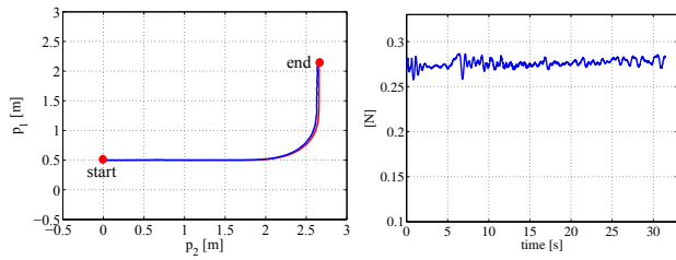
(a) Path (p_1, p_2) : desired position (red), actual position (blue).
