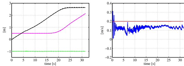
(c) Positions: p_1(t) (magenta), p_2(t) (black), p_3(t) (green); dashed lines are desired positions, while solid lines are actual positions.
