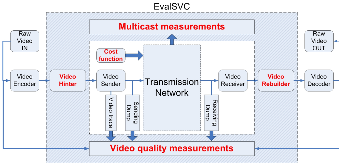
Fig. 3 EvalSVC: An evaluation platform of SVC-based services.
