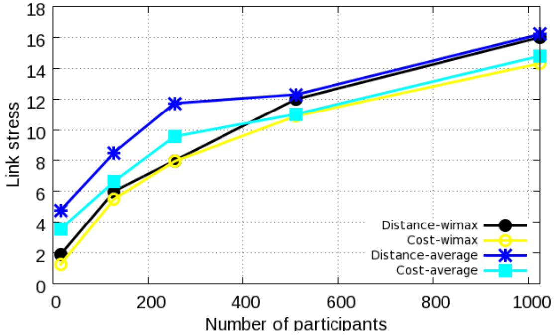
Fig. 12 Link stress performance of the video conferencing service built over a convergent underlay network comprised of a simulated Internet topology and a real mobile WiMAX network.
