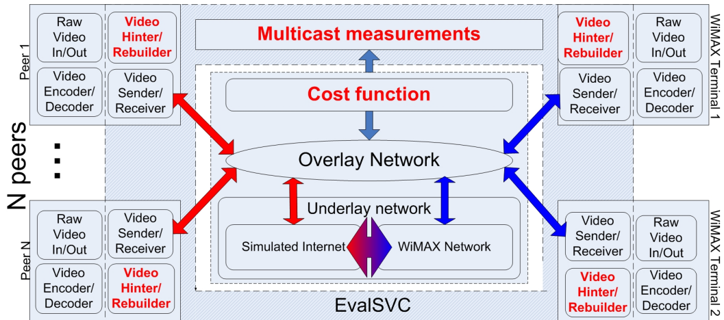
Fig. 11 Performance evaluation platform of SVC-based conferencing services on the overlay network built over a convergent underlay network comprised of a simulated Internet topology and a real mobile WiMAX network. The Application Layer Multicast tree is constructed using the newly proposed cross-layer multi-variable cost function.
