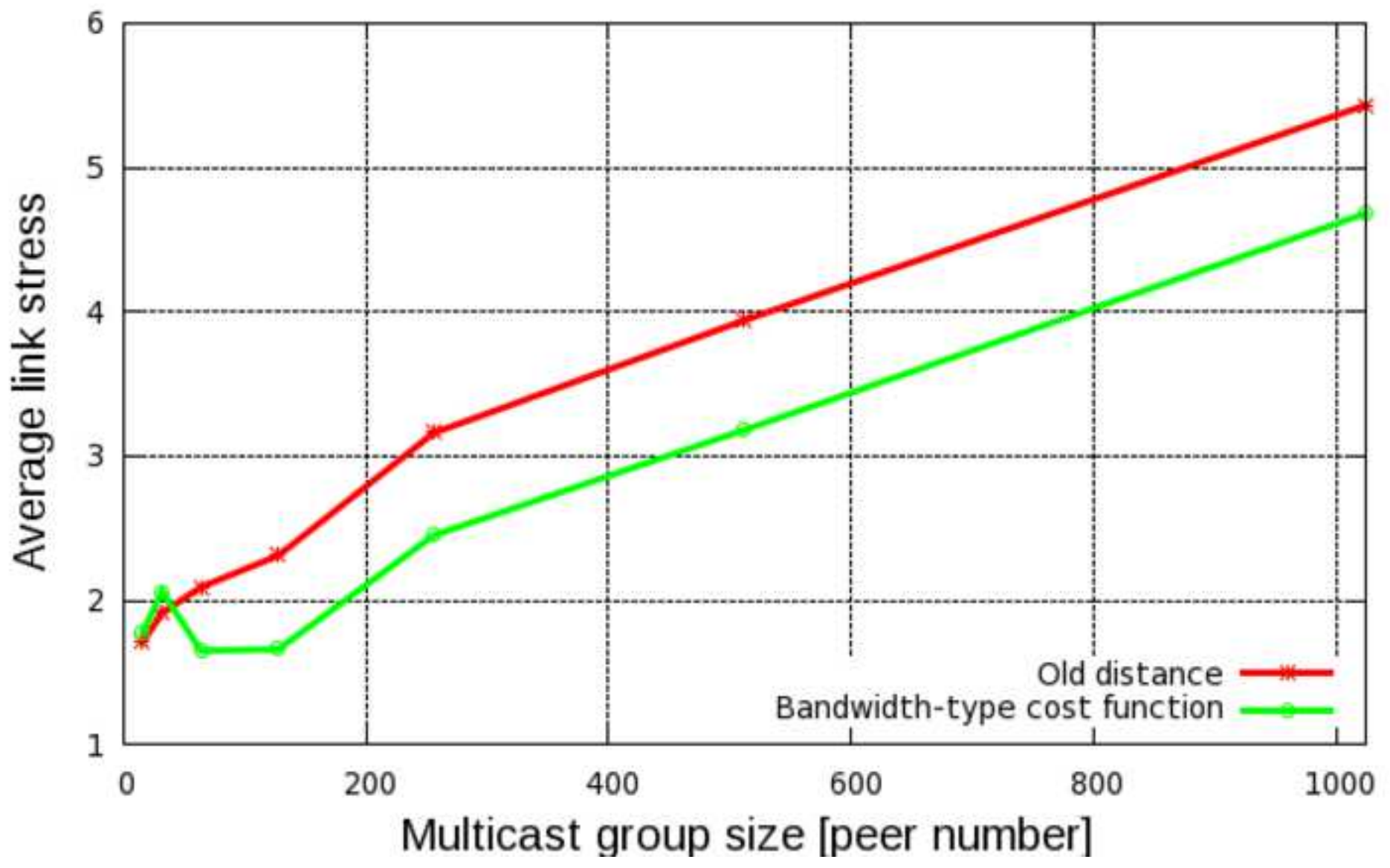
Average link stress for distance and bandwidth-type cost function
