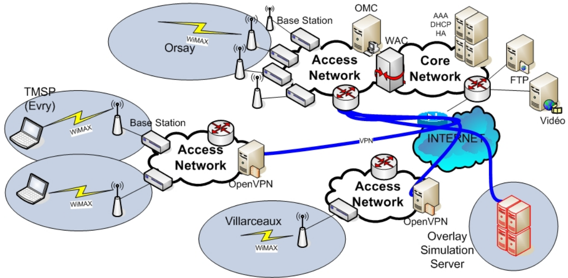
Fig. 9 Convergent underlay network composed of real POSEIDON's Alcatel-Lucent mobile WiMAX network and an overlay simulation platform [1].
