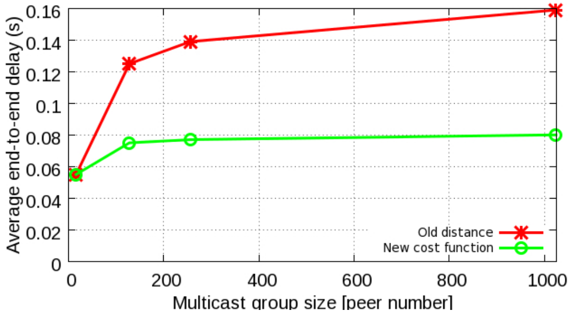
Fig. 8 Average end-to-end delay comparison for the NICE data-plan using the old and new cost functions. Transmitting data is obtained from a real SVC multicast session.
