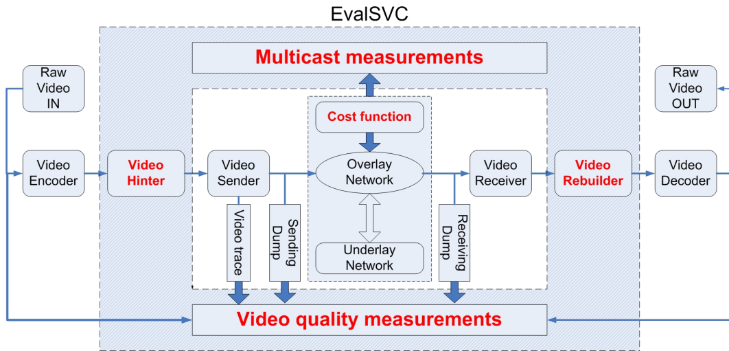
Fig. 5 Performance evaluation platform of SVC-based multicast service on an overlay network constructed from our newly proposed cross-layer multi-variable cost function.
