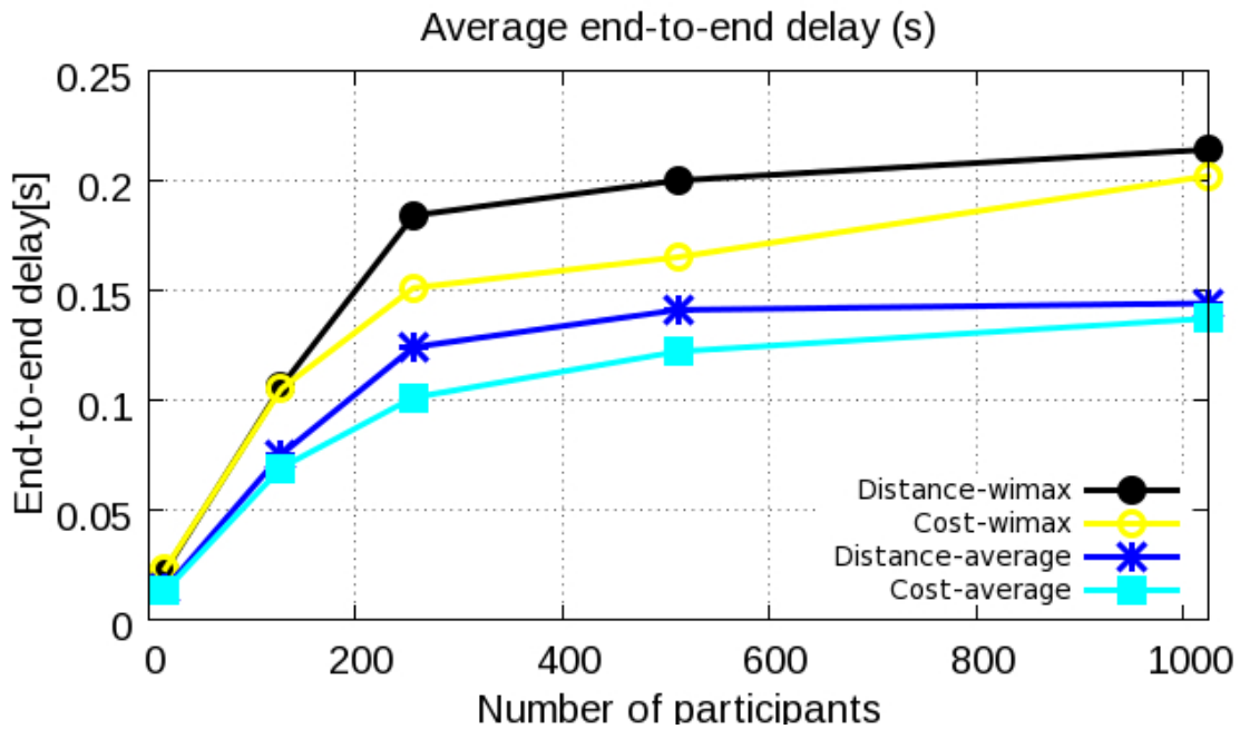
Fig. 13 End to end delay performance of the video conferencing service built over a convergent underlay network comprised of a simulated Internet topology and a real mobile WiMAX network.
