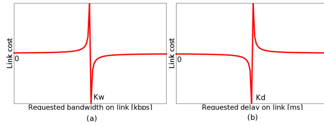
Fig. 1 Bandwidth-type (a) and delay-type (b) cost functions according to Equ.11 and Equ.13.
