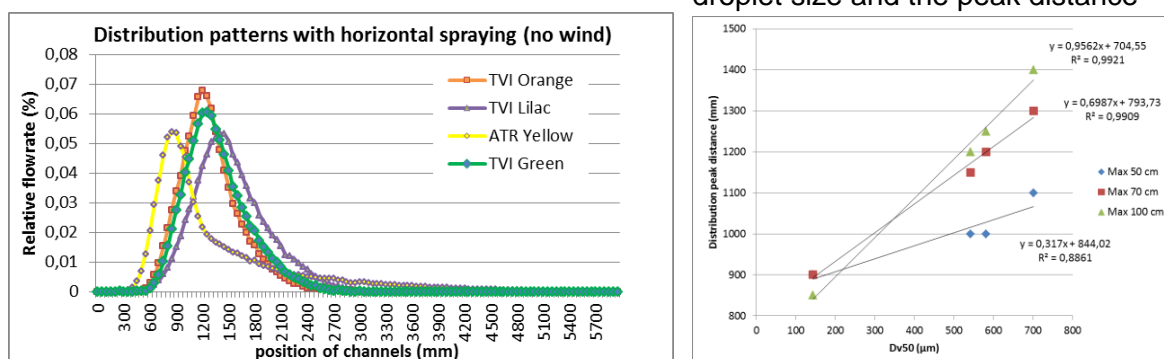
Fig 1a and 1b: Distribution patterns form horizontal spraying (1 m height) and correlation between droplet size and the peak distance
