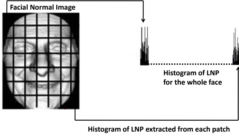
Figure 7: Illustration of facial normal representation: histogram of LNP.
